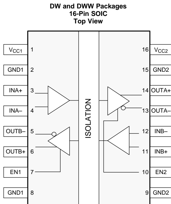
Pin Functions
