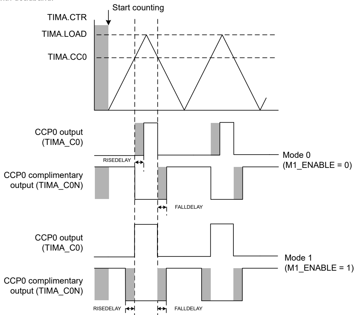
Figure 24-33. Dead Band Insertion for Center-Aligned PWM (Mode 0 and Mode 1)
