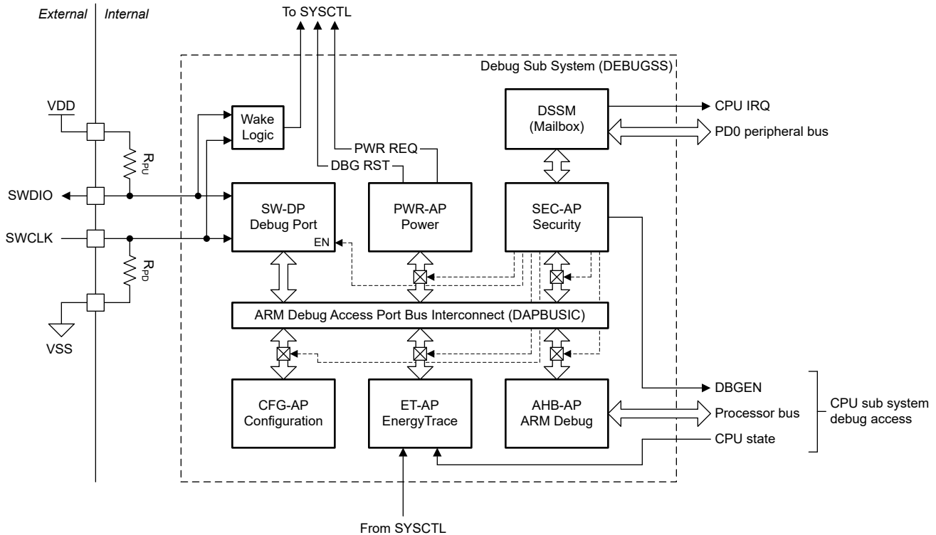
Figure 30-1. Debug Sub System Block Diagram
