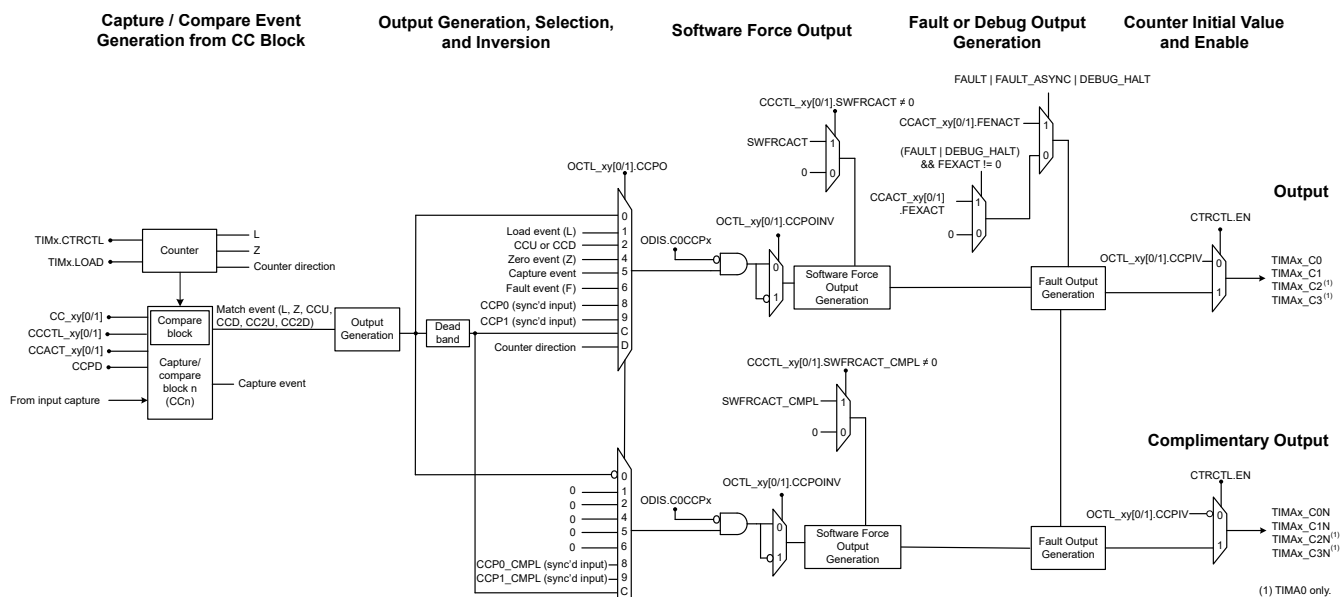
Figure 24-27. Output Connection for TIMA
