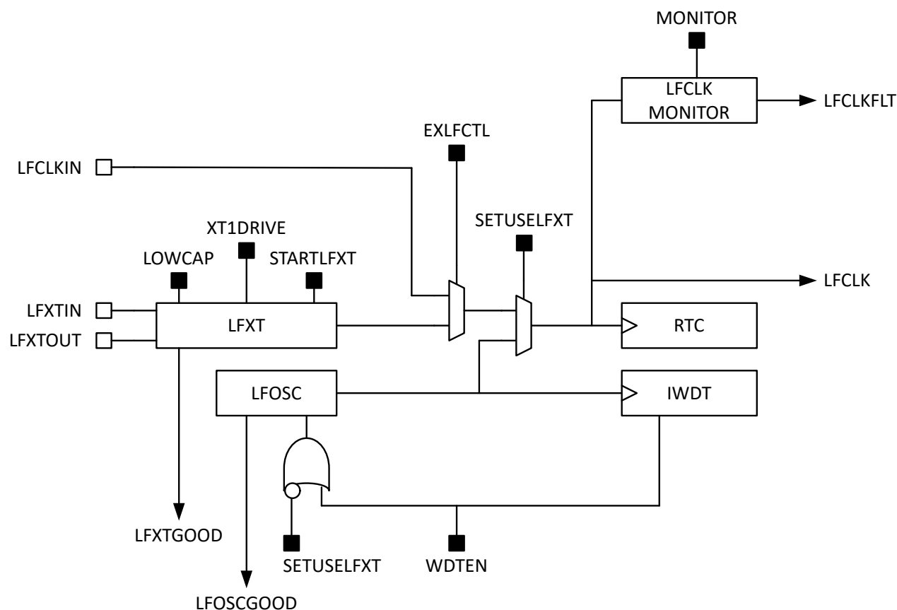
Figure 26-1. LFSS Low-Frequency Clock System
