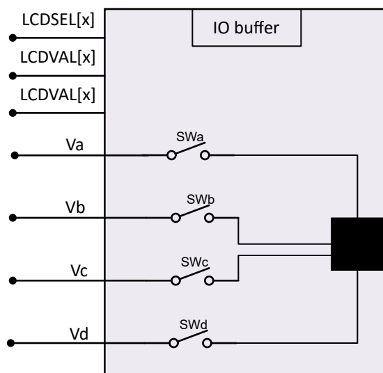
Figure 20-35. IO Muxing
