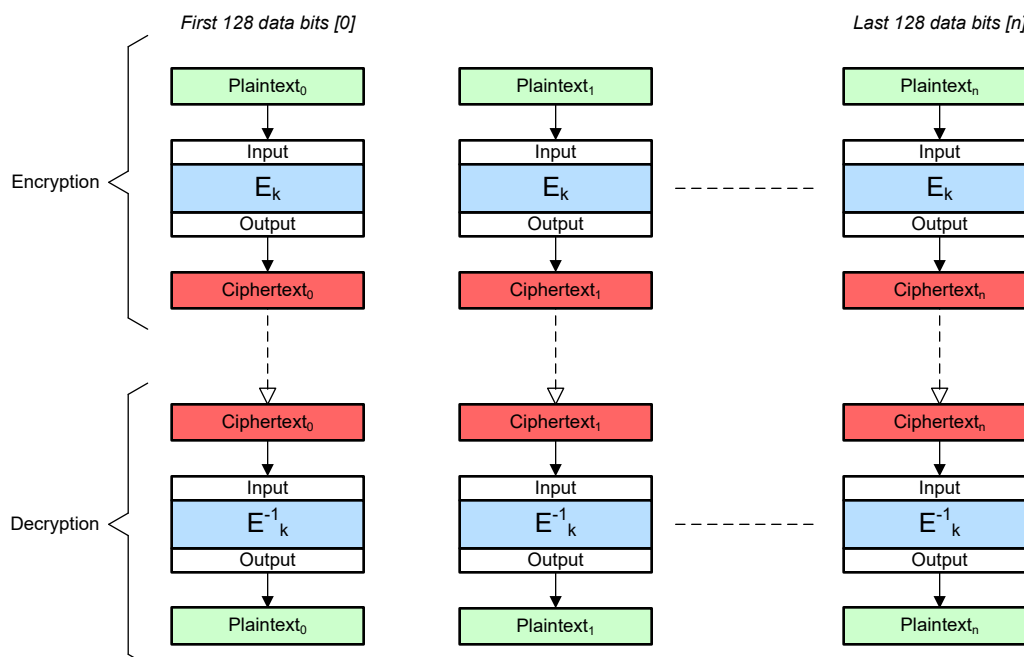
Figure 10-2. ECB Cipher
