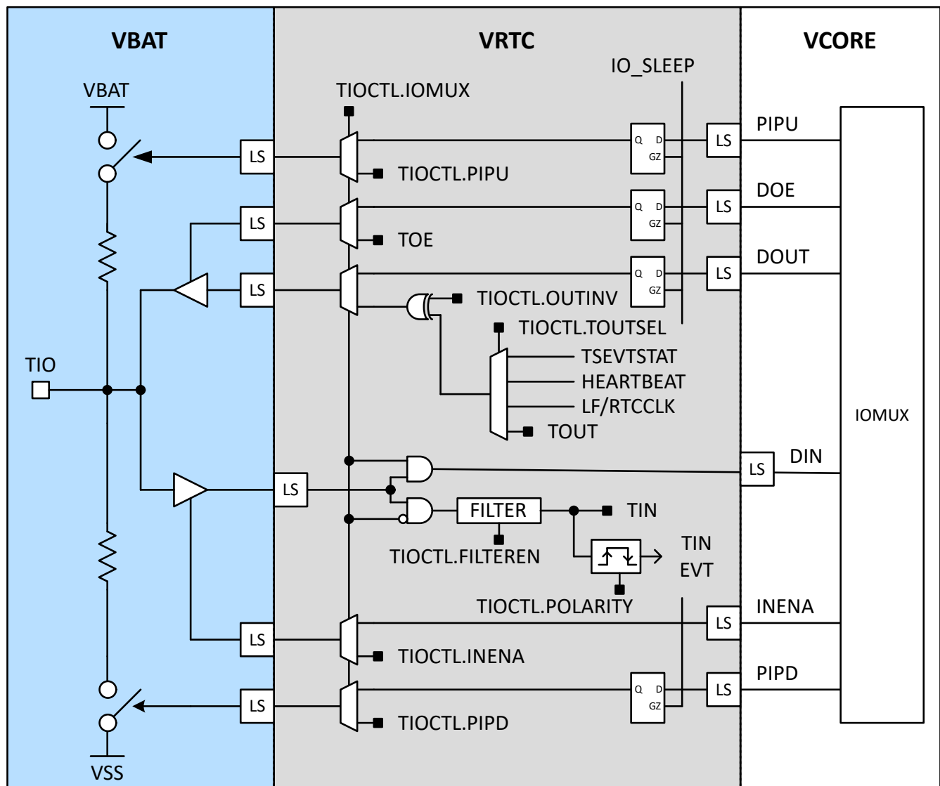
Figure 25-5. Tamper I/O Circuit Diagram
