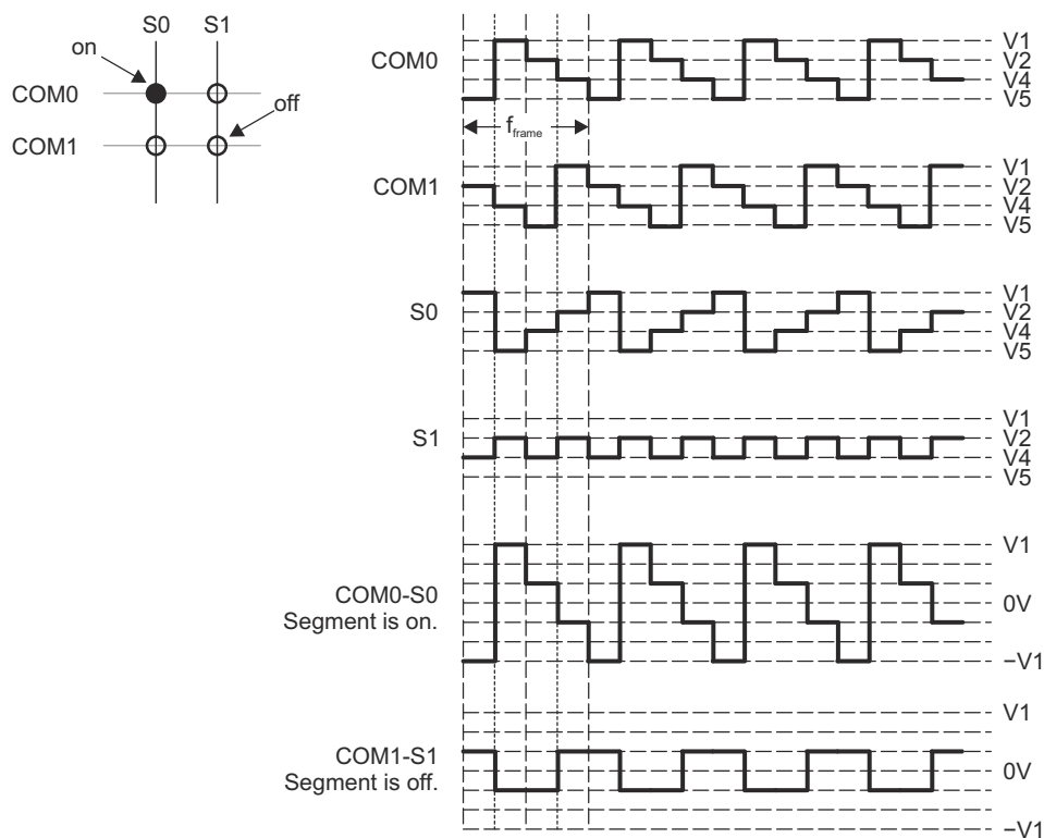
Figure 20-3. Example 2-Mux Waveforms
