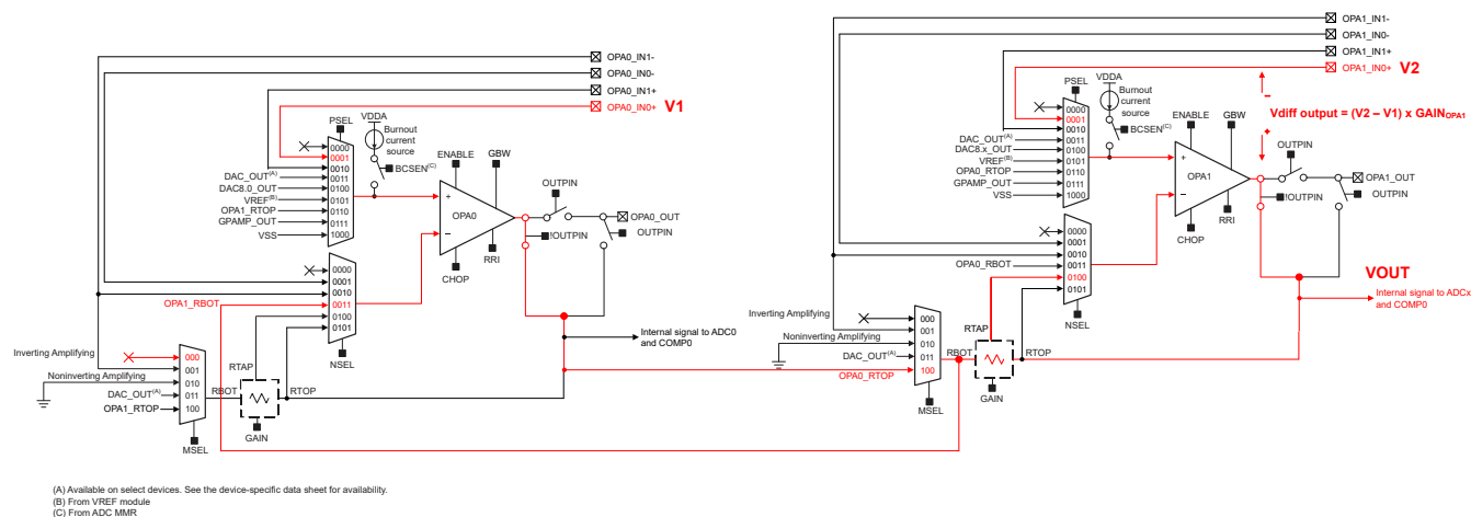
Figure 17-8. Two OPAs in Difference Amplifier Configuration
