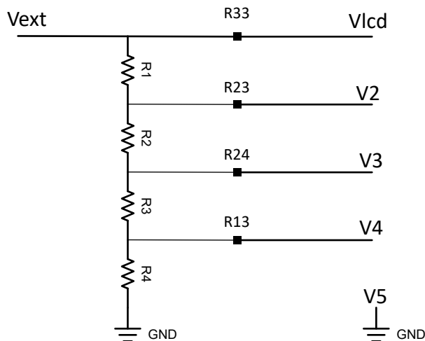
Figure 20-12. Voltage Generation in Mode 0
