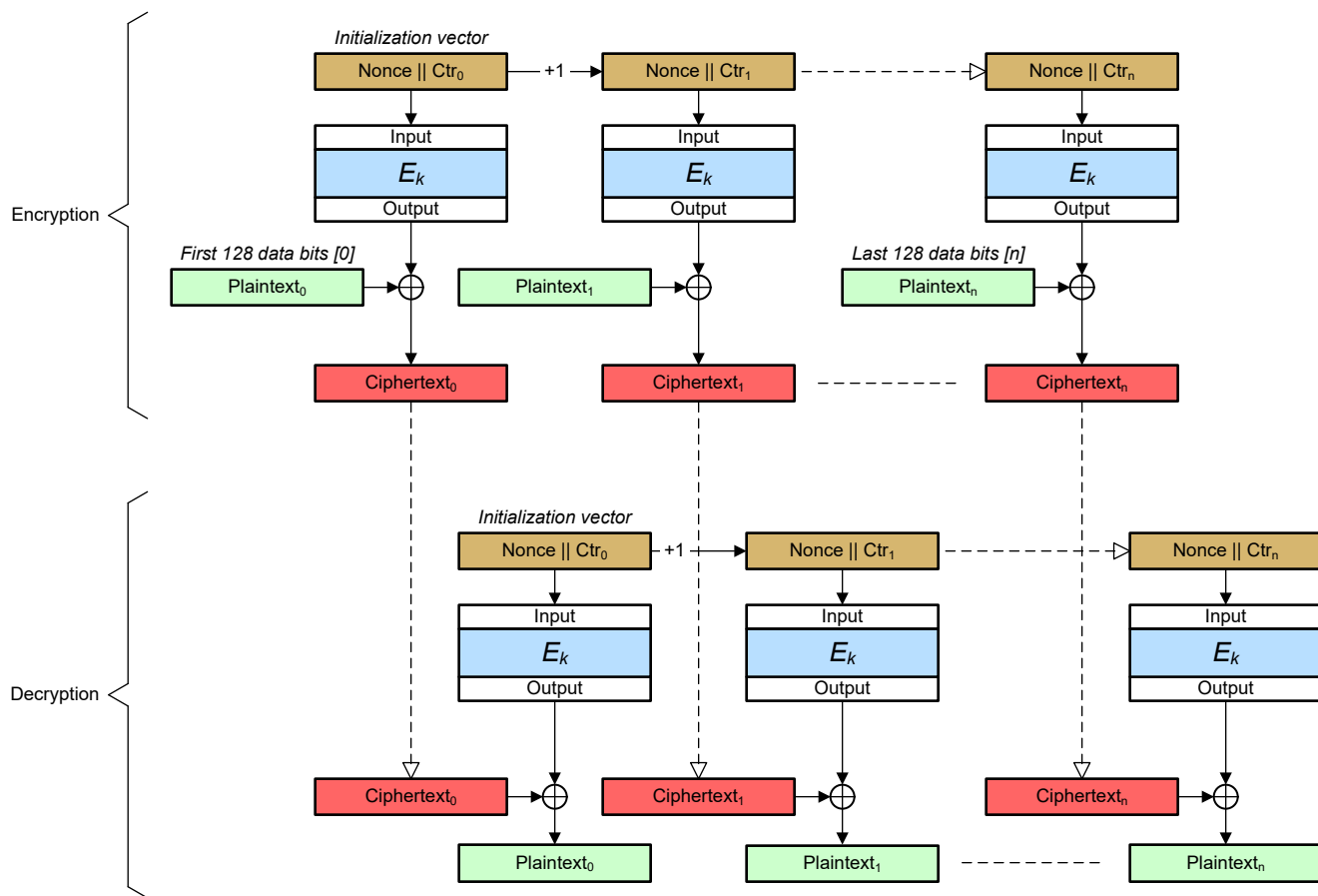
Figure 10-6. CTR Cipher
