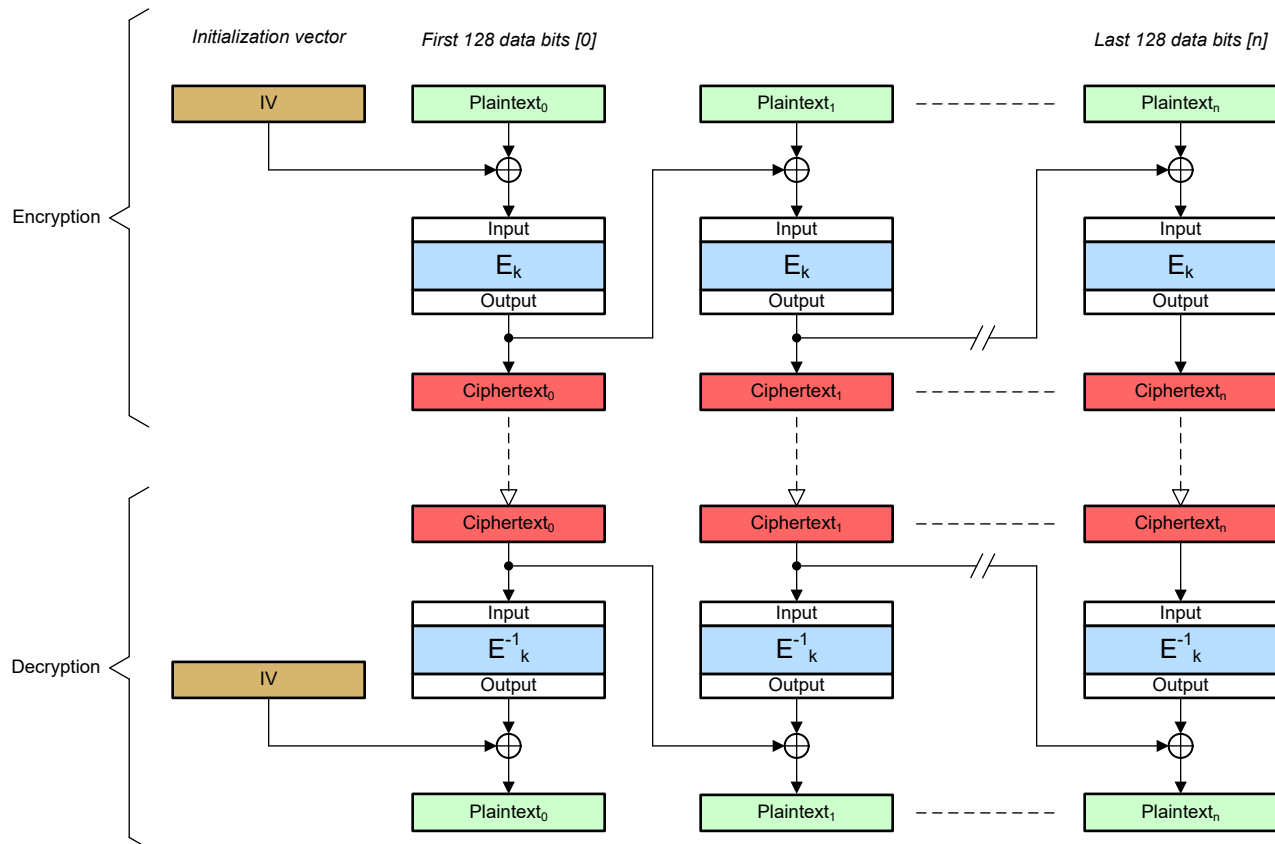
Figure 10-3. CBC Cipher
