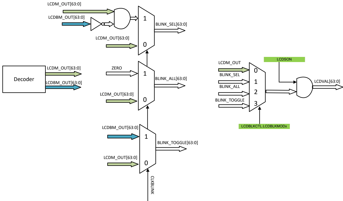
Figure 20-34. Blinking override
