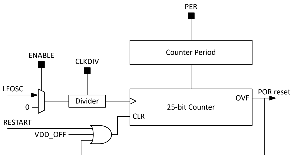
Figure 28-1. Independent Watchdog Timer (IWDT) Block Diagram
