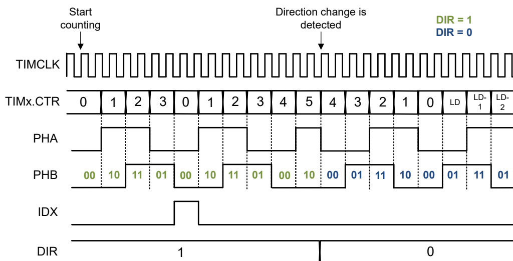
Figure 24-20. 2-Signal QEI with Index Input Operation
