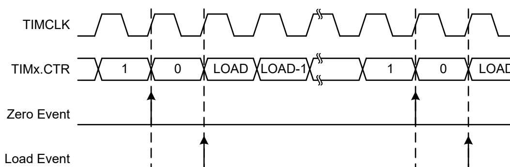
Figure 24-6. Down Counting Mode Event Generation
