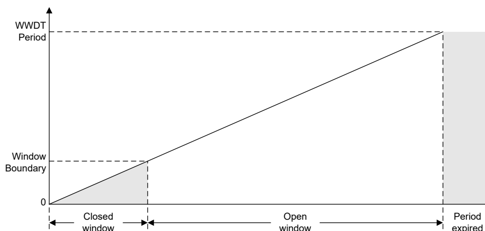
Figure 29-1. WWDT Functionality
