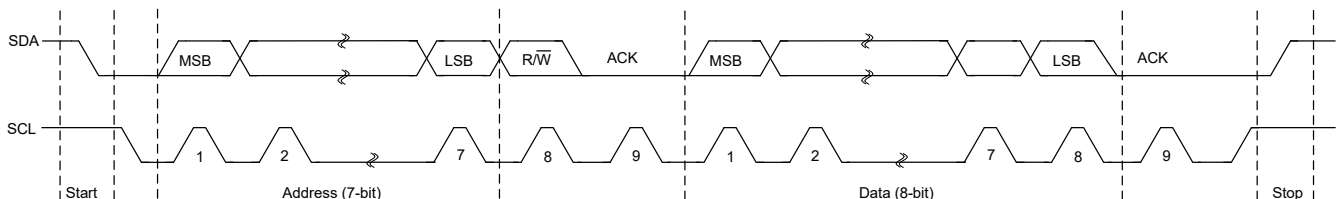
Figure 22-3. Module Data Transfer
