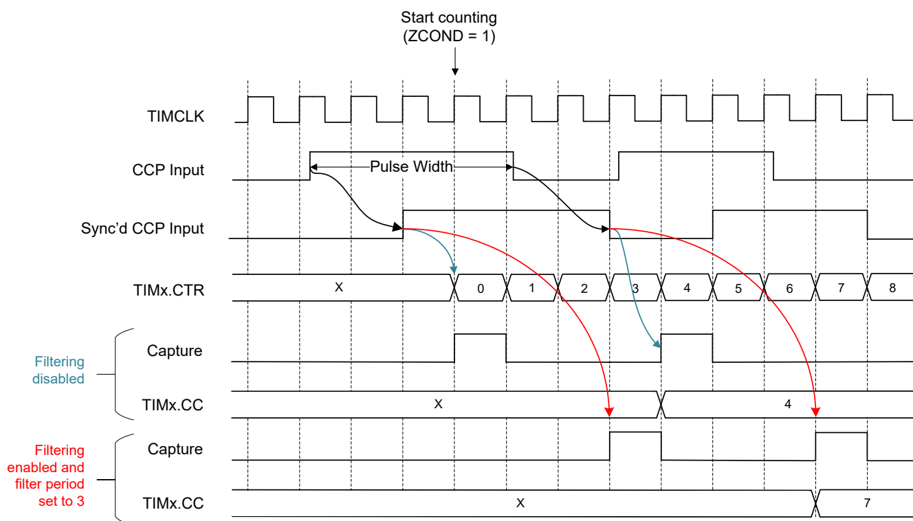
Figure 24-16. Pulse-Width Capture Mode
