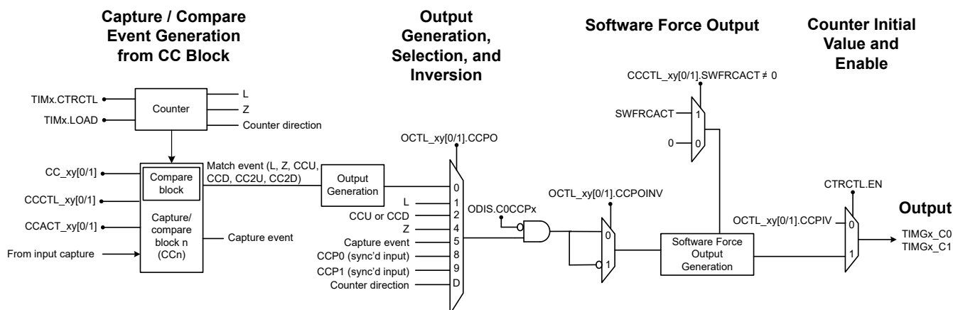
Figure 24-26. Output Connection for TIMG
