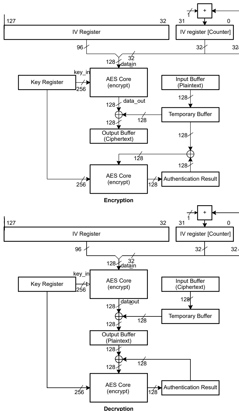
Figure 10-10. CCM Operation
