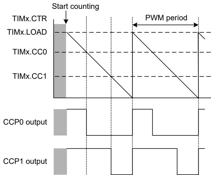
Figure 24-28. Edge-Aligned PWM Signals in Down-Counting Mode
