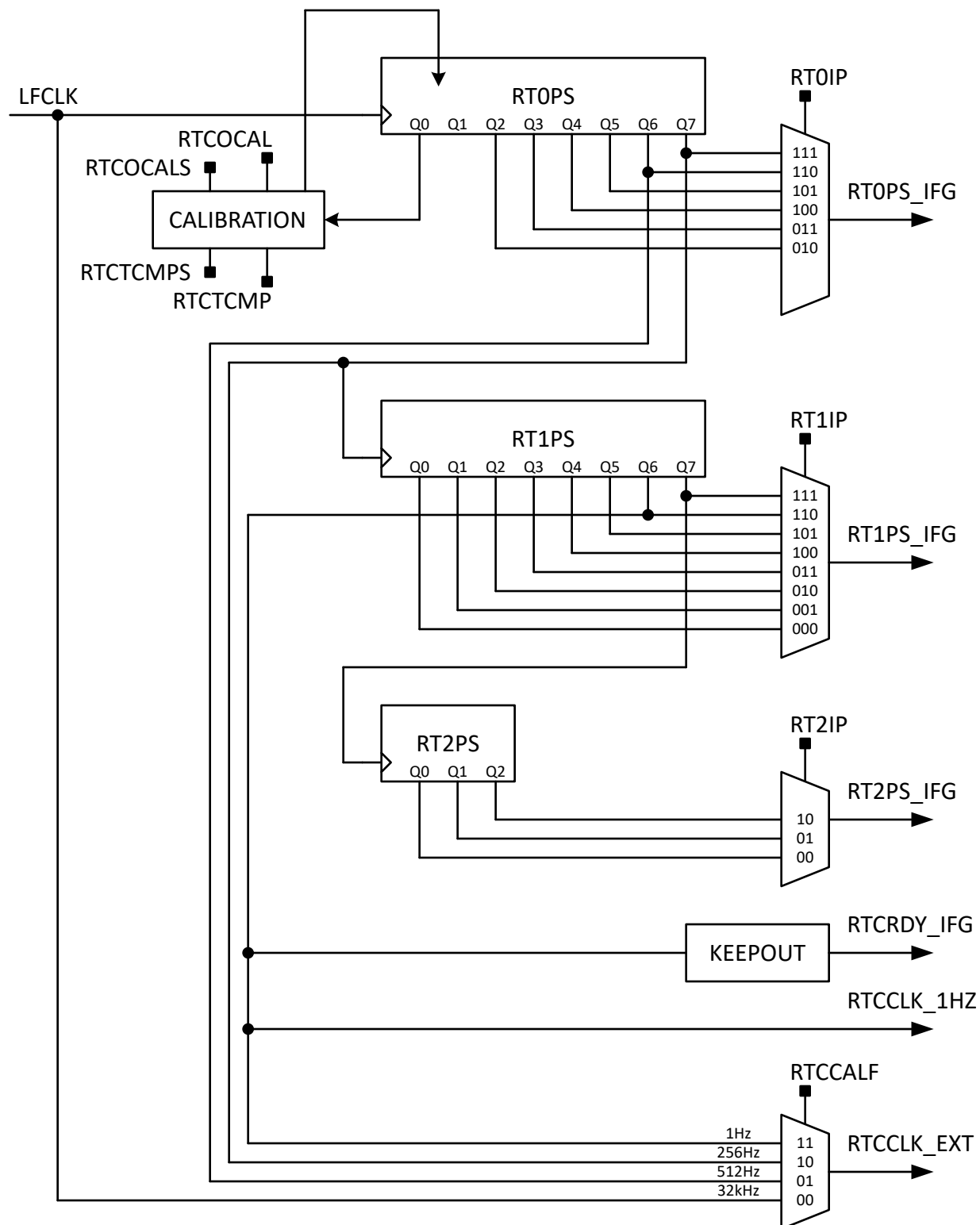
Figure 27-3. RTC Prescaler and Interval Timer Event
