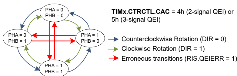
Figure 24-18. State Machine for 2-signal and 3-signal QEI mode
