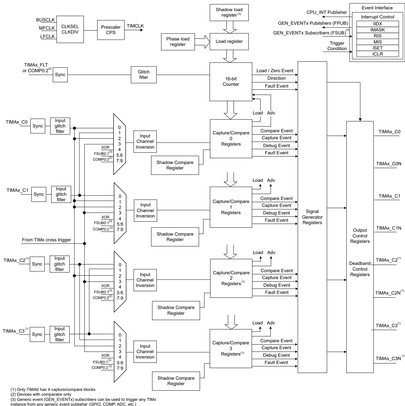
Figure 24-2. TIMA Block Diagram
