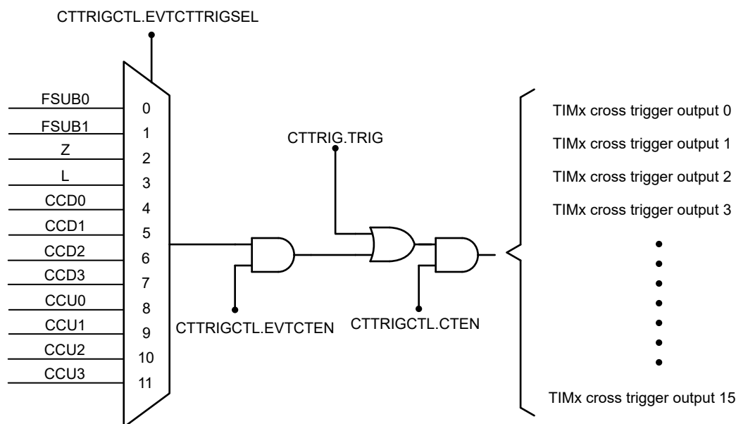
Figure 24-39. Main Timer Cross Trigger Output Configuration
