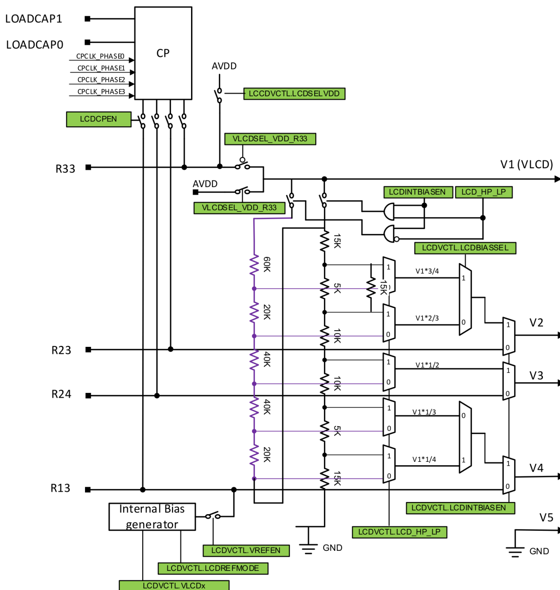
Figure 20-11. LCD Clocks
