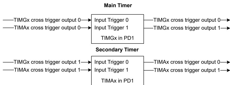
Figure 24-38. Cross Trigger Connections for Main Timer (TIMGx) and Secondary Timer (TIMAx) in Power Domain 1
