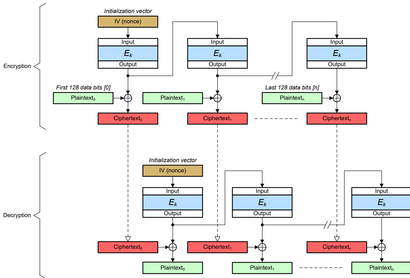
Figure 10-4. OFB Cipher
