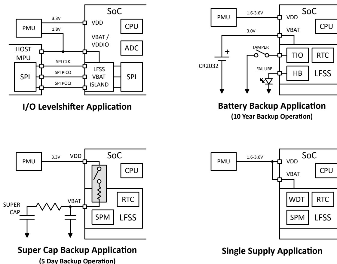
Figure 25-3. LFSS Typical Application Use Cases
