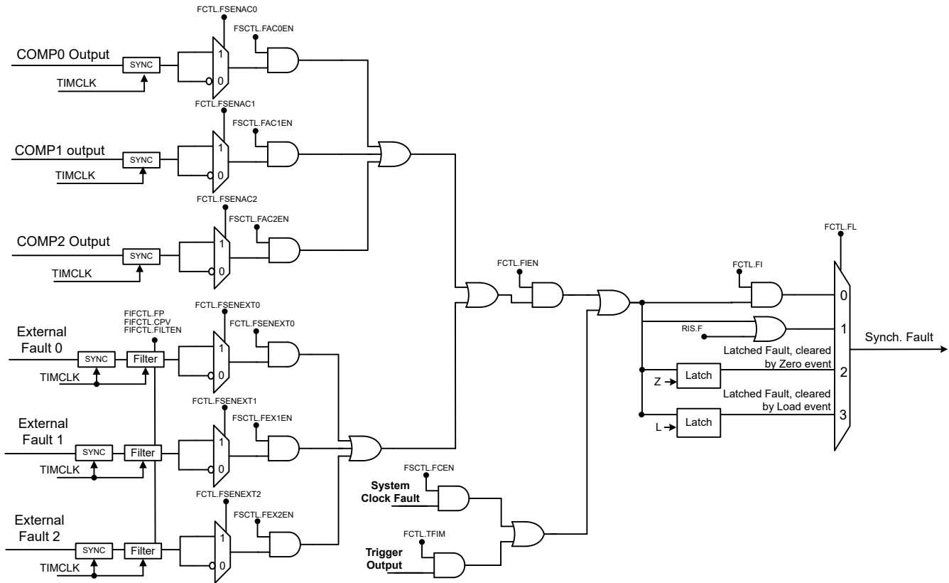
Figure 24-35. Synchronous Fault Handler Connections
