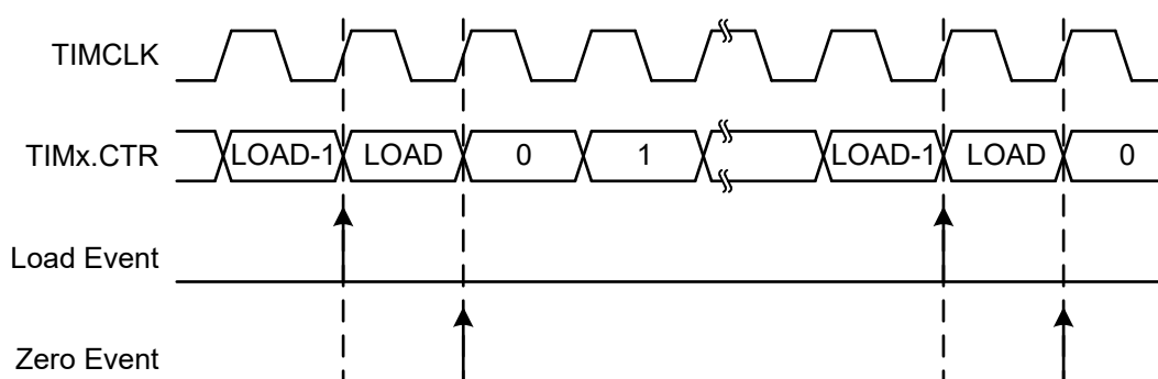
Figure 24-10. Up Counting Mode Event Generation
