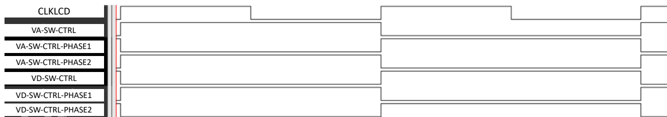
Figure 20-24. Switch Control Signals - Static Mode
