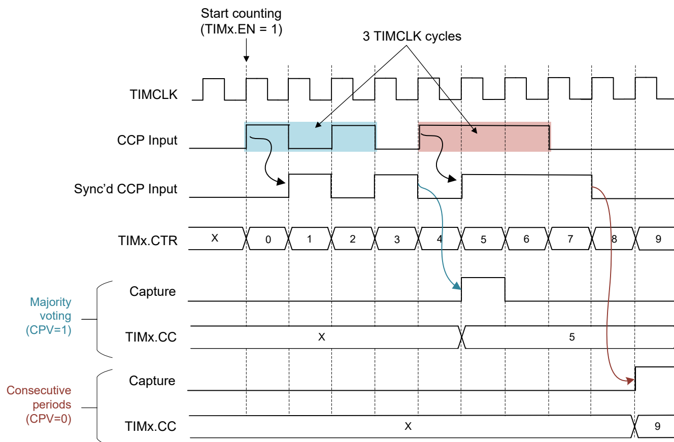
Figure 24-13. Consecutive Period and Majority Voting for Input Glitch Filtering using FP = 0 (3 TIMCLK cycles)
