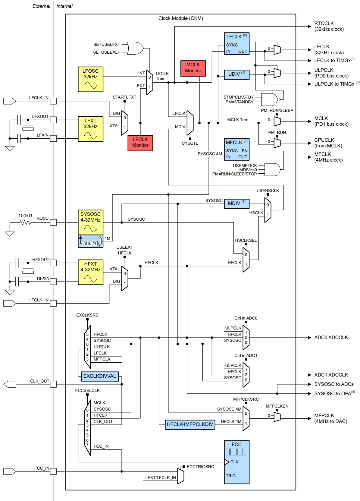
Figure 2-7. MSPM0Lxx Top Level Clock Tree
