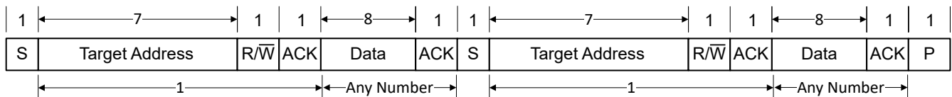
Figure 22-7. Data Format with Repeated Start
