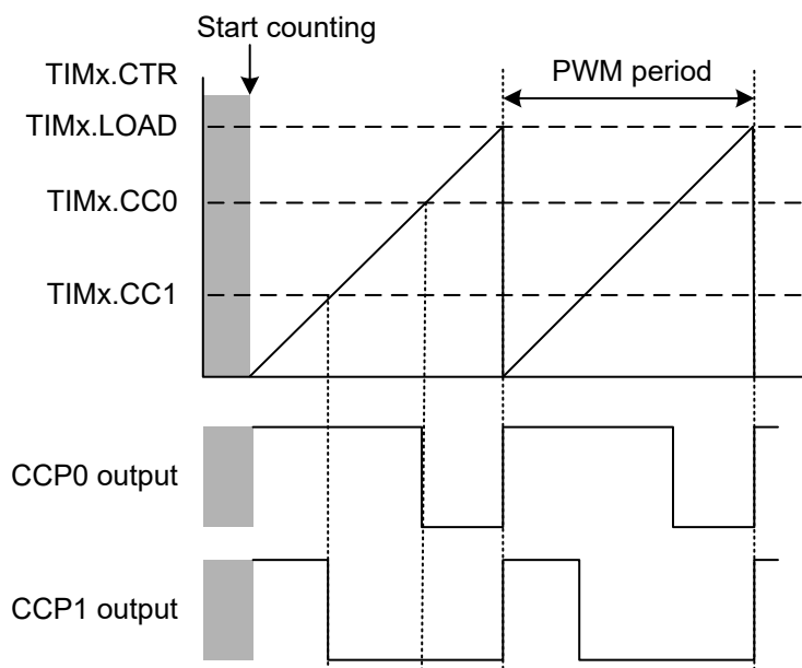
Figure 24-29. Edge-Aligned PWM Signals in Up-Counting Mode
