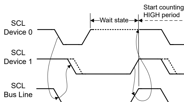
Figure 22-9. Clock Synchronization
