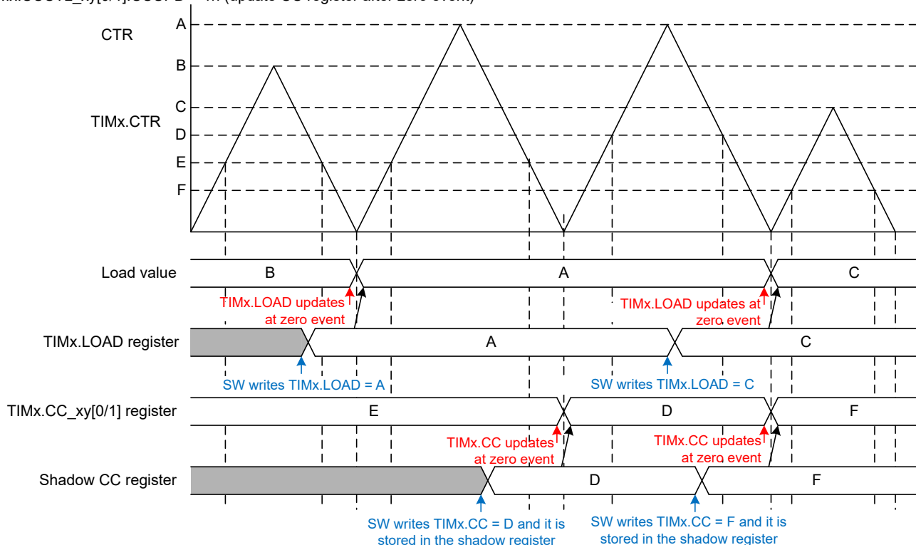
Figure 24-25. Shadow Load and Shadow Compare Taking Effect at Zero Event in Up/Down Mode
