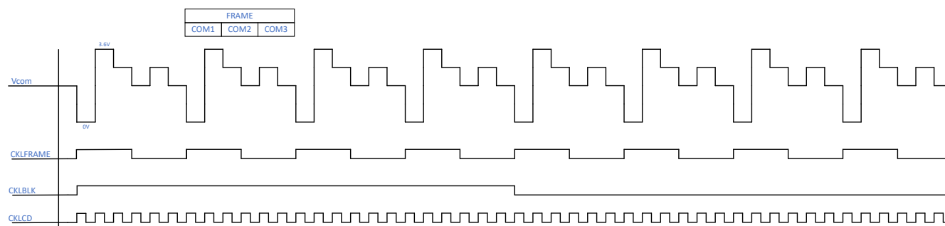
Figure 20-10. CLKLCD, CLKFRAME, and CLKBK Relationship
