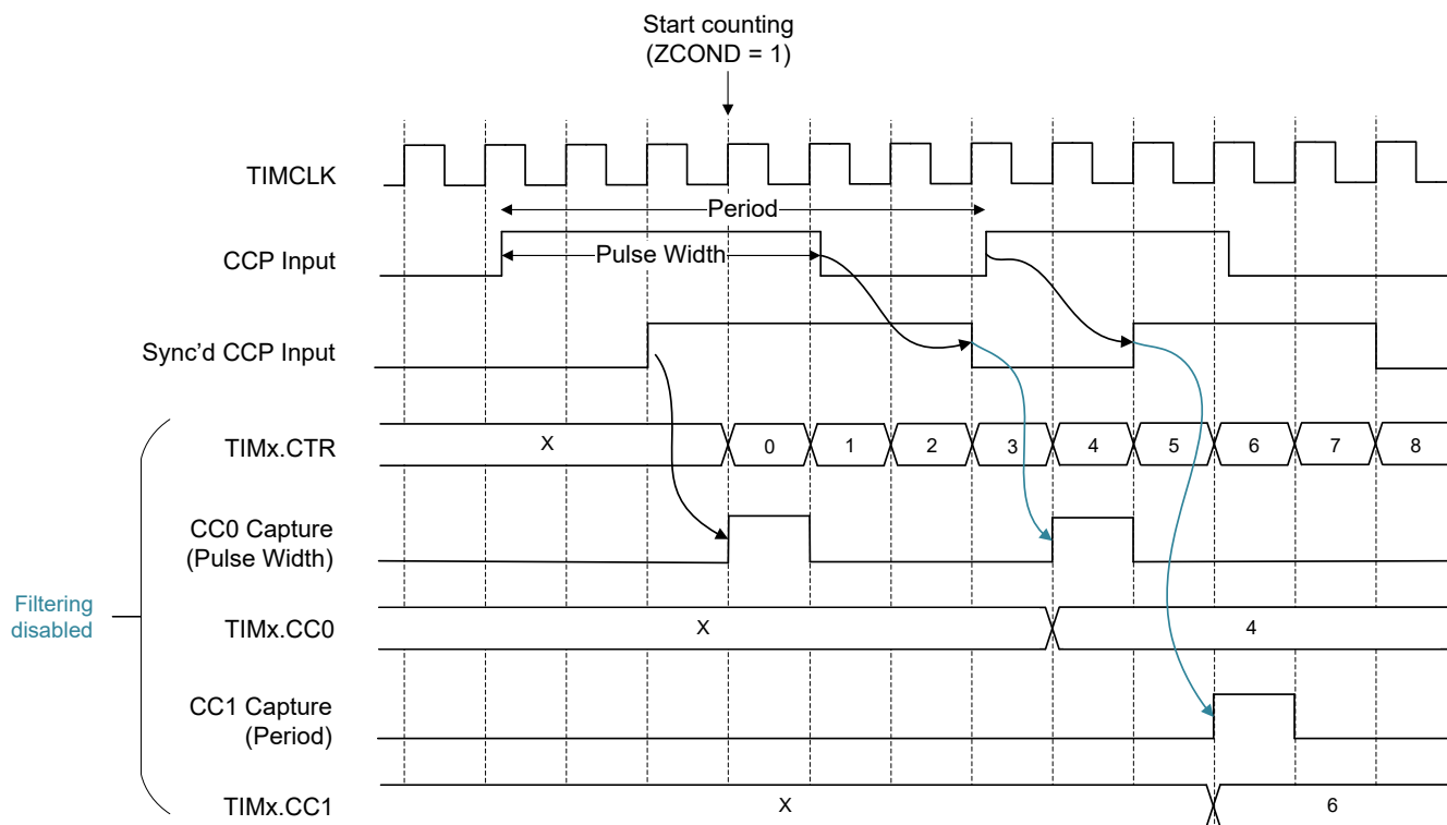
Figure 24-17. Combined Pulse-Width and Period Capture
