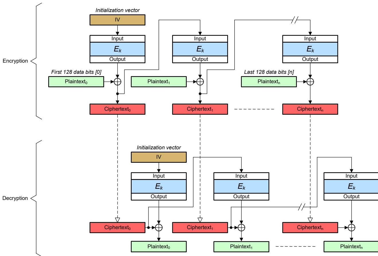
Figure 10-5. CFB Cipher
