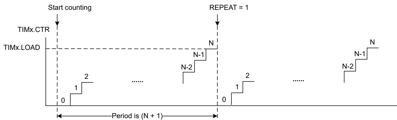
Figure 24-9. Up Counting Mode, CVAE = 2
