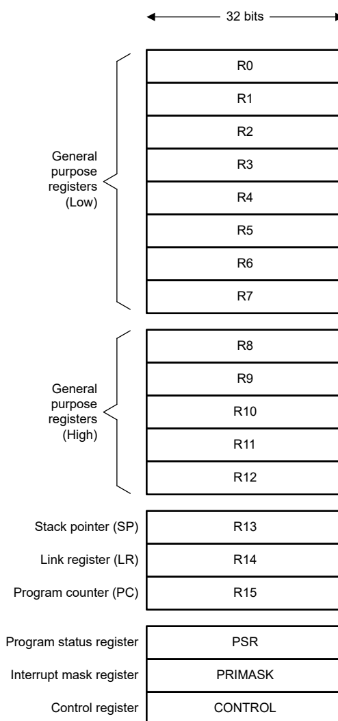
Figure 3-2. CPU Registers
