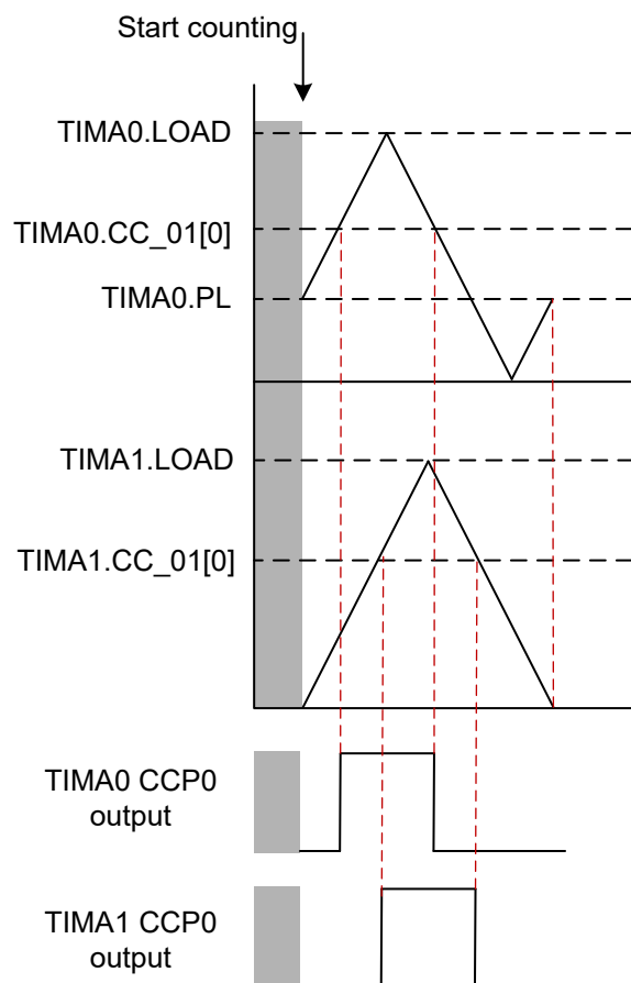
Figure 24-31. Asymmetric PWM Configuration with Phase Load for CCP channel 0 of TIMA0 and TIMA1
