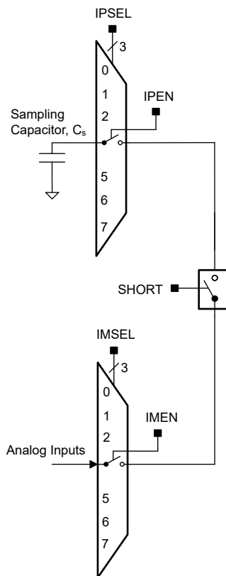
Figure 16-4. Comparator Short Switch
