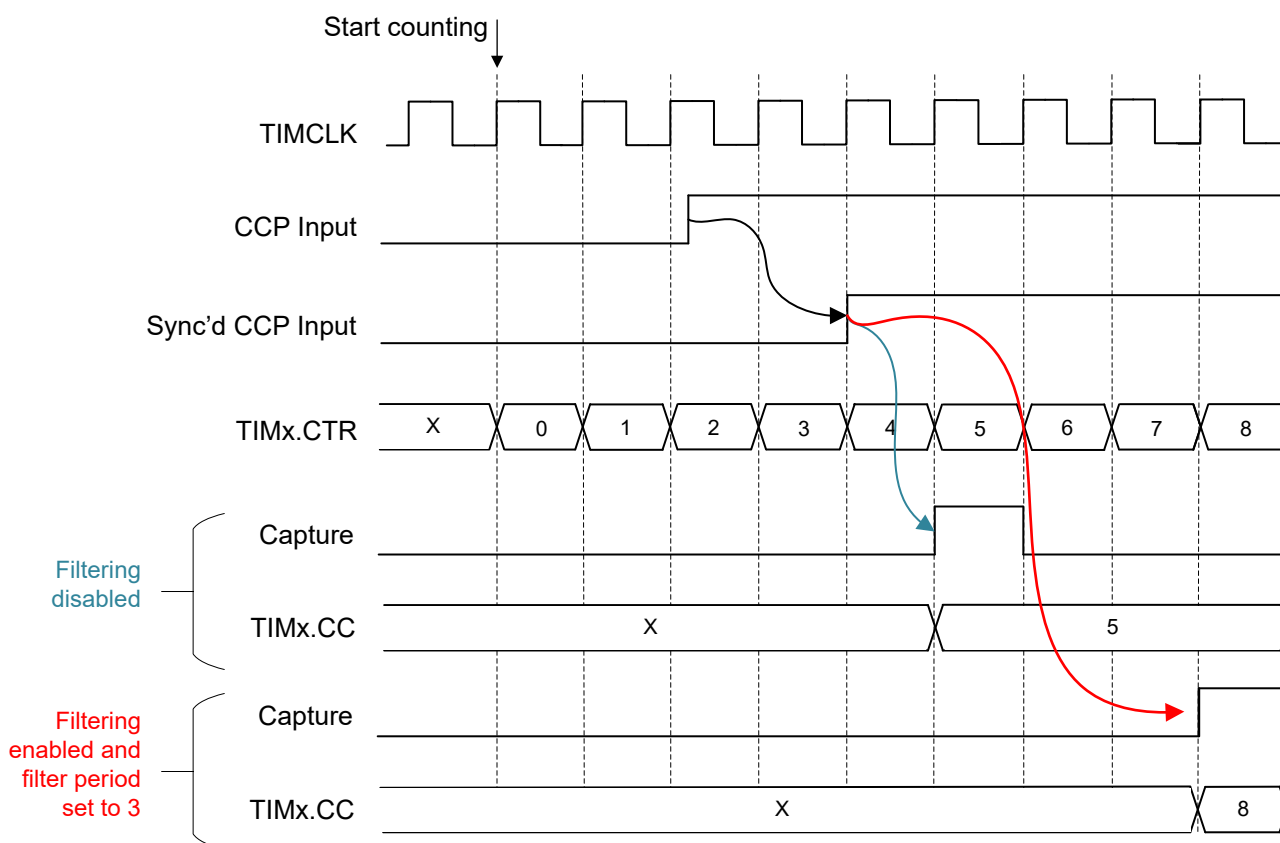
Figure 24-14. Edge Time Capture Mode in Up-Counting Mode, CVAE = 2
