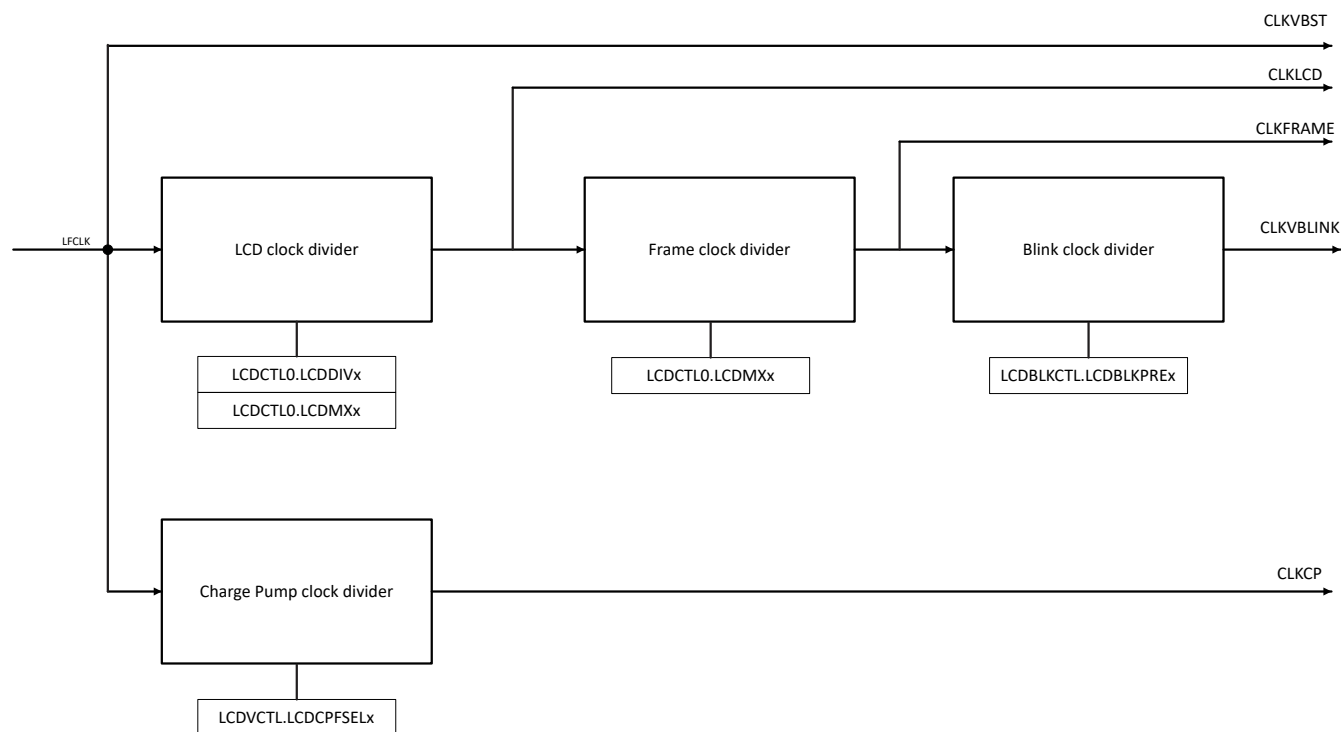
Figure 20-9. LCD Clocks
