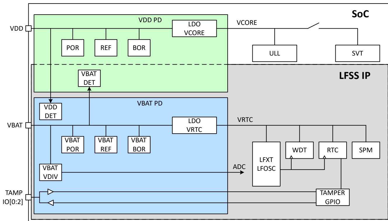
Figure 25-1. LFSS Overview
