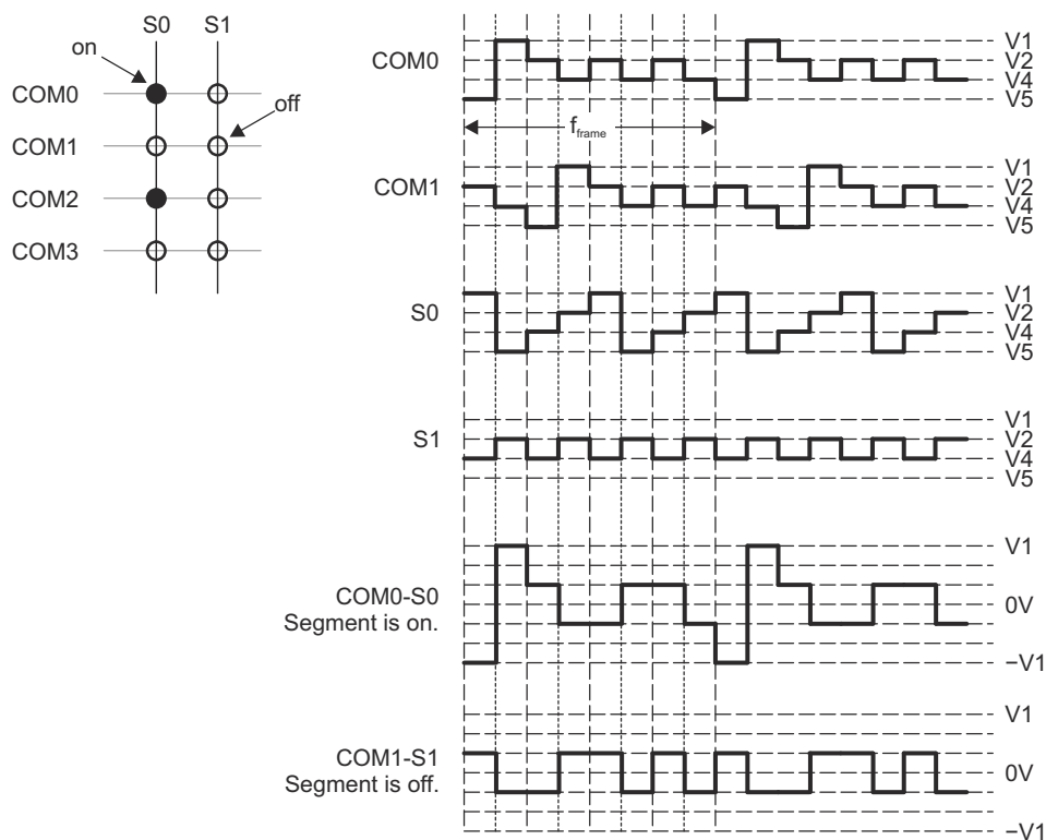
Figure 20-5. Example 4-Mux Waveforms
