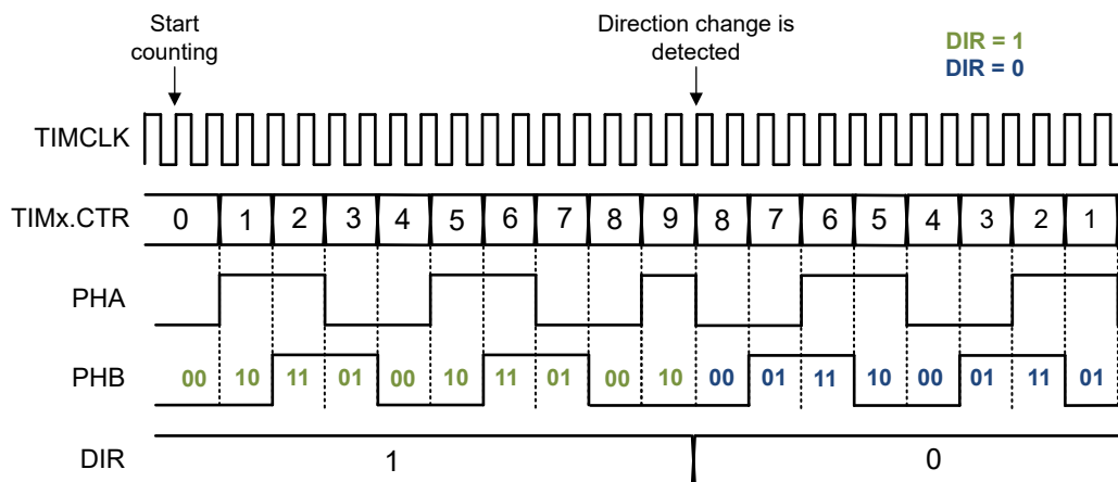
Figure 24-19. 2-Signal QEI Operation
