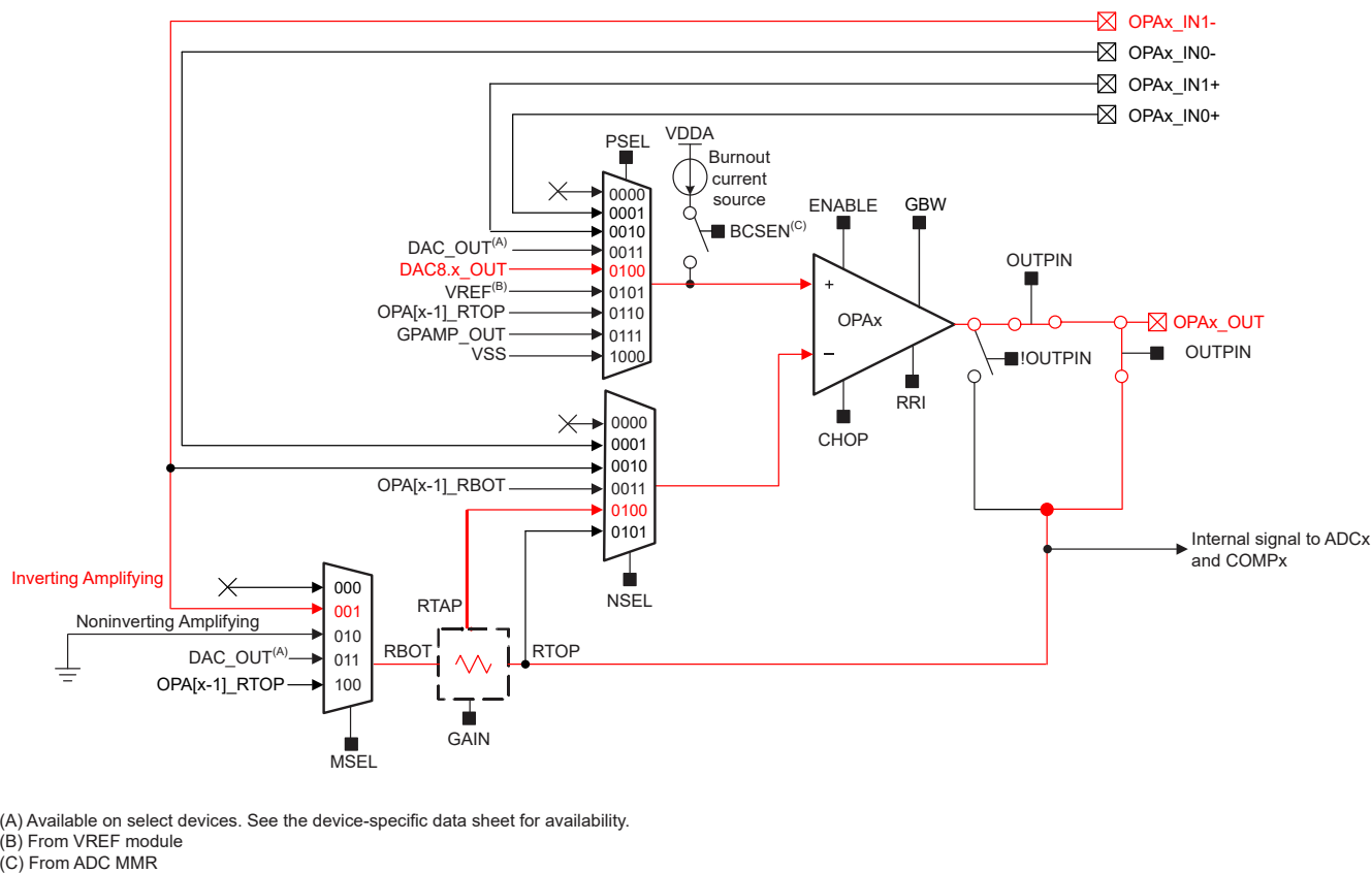
Figure 17-5. OPA in Inverting PGA Configuration
