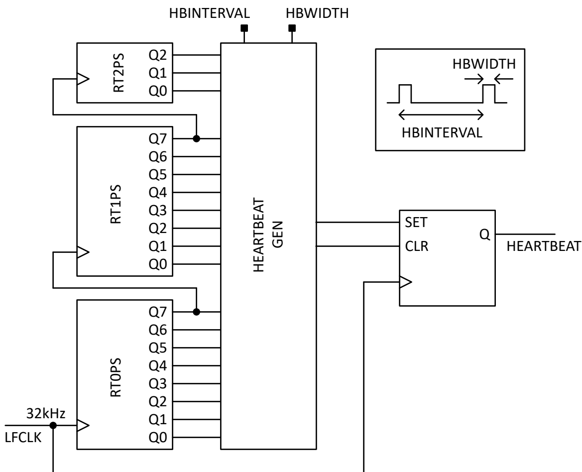
Figure 25-6. Heartbeat Generator Circuit Diagram
