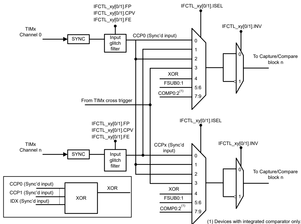
Figure 24-12. TIMx Capture Block Diagram
