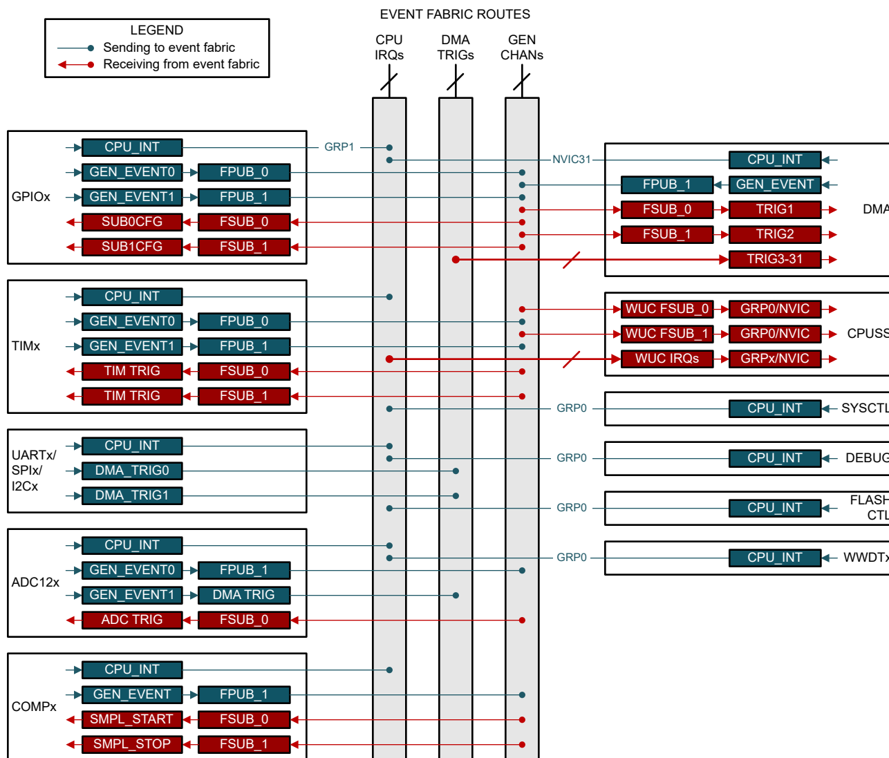
Figure 7-5. Event Map
