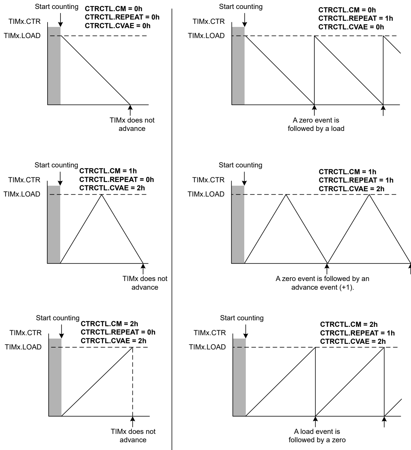
Figure 24-4. One-shot and Periodic Mode Behavior
