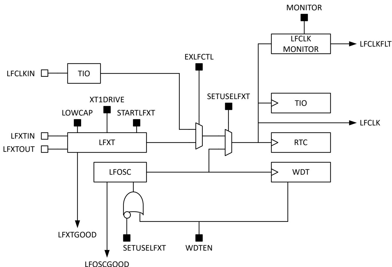
Figure 25-2. LFSS Low-Frequency Clock System
