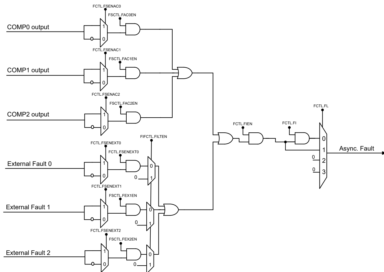
Figure 24-34. Asynchronous Fault Handler Connections
