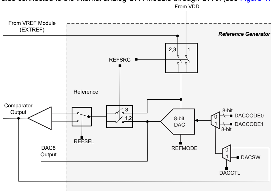
Figure 16-3. Reference Voltage Generator Block Diagram
