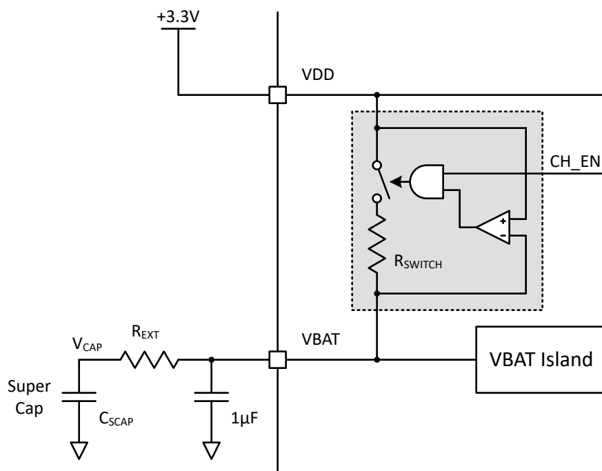
Figure 25-4. Supercapacitor Charging Circuit
