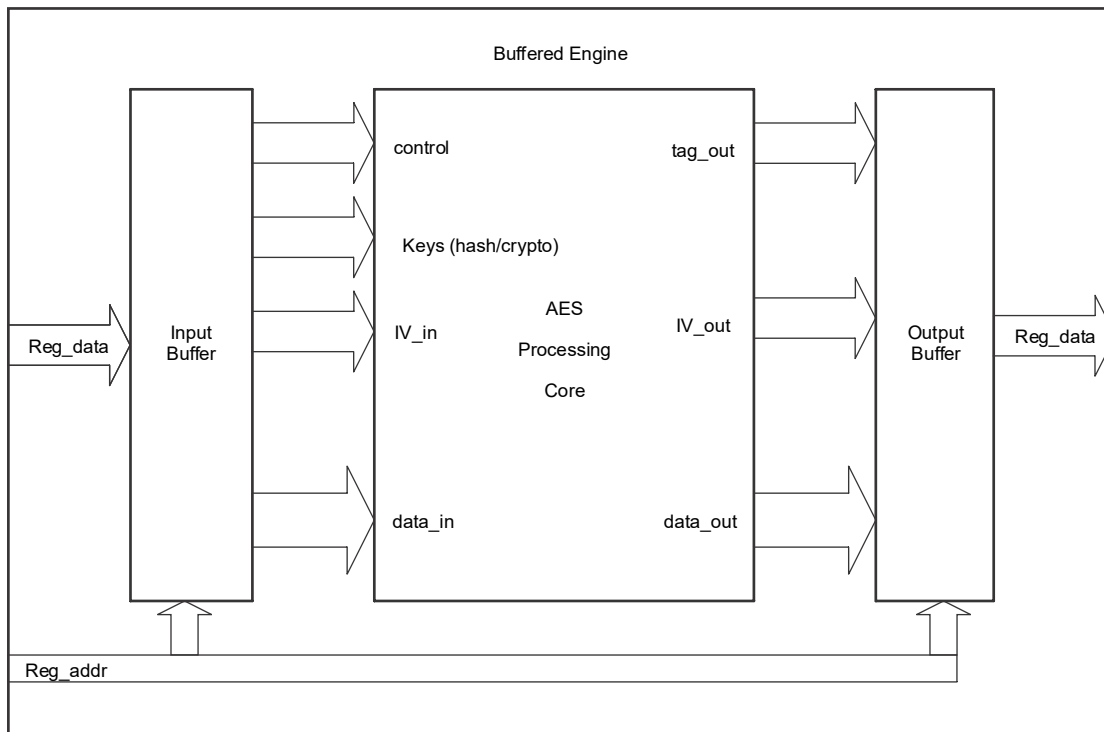
Figure 10-1. AESADV Block Diagram
