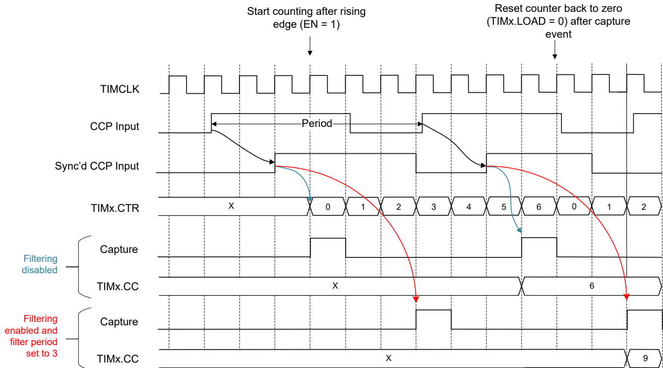
Figure 24-15. Period Capture Mode in Up-Counting Mode, CVAE = 2
