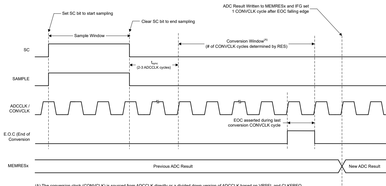
Figure 15-4. MANUAL Sampling Mode ADC Sample and Conversion Timing Diagram
