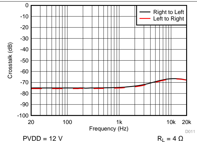
Figure 16. Crosstalk vs Frequency - BTL
