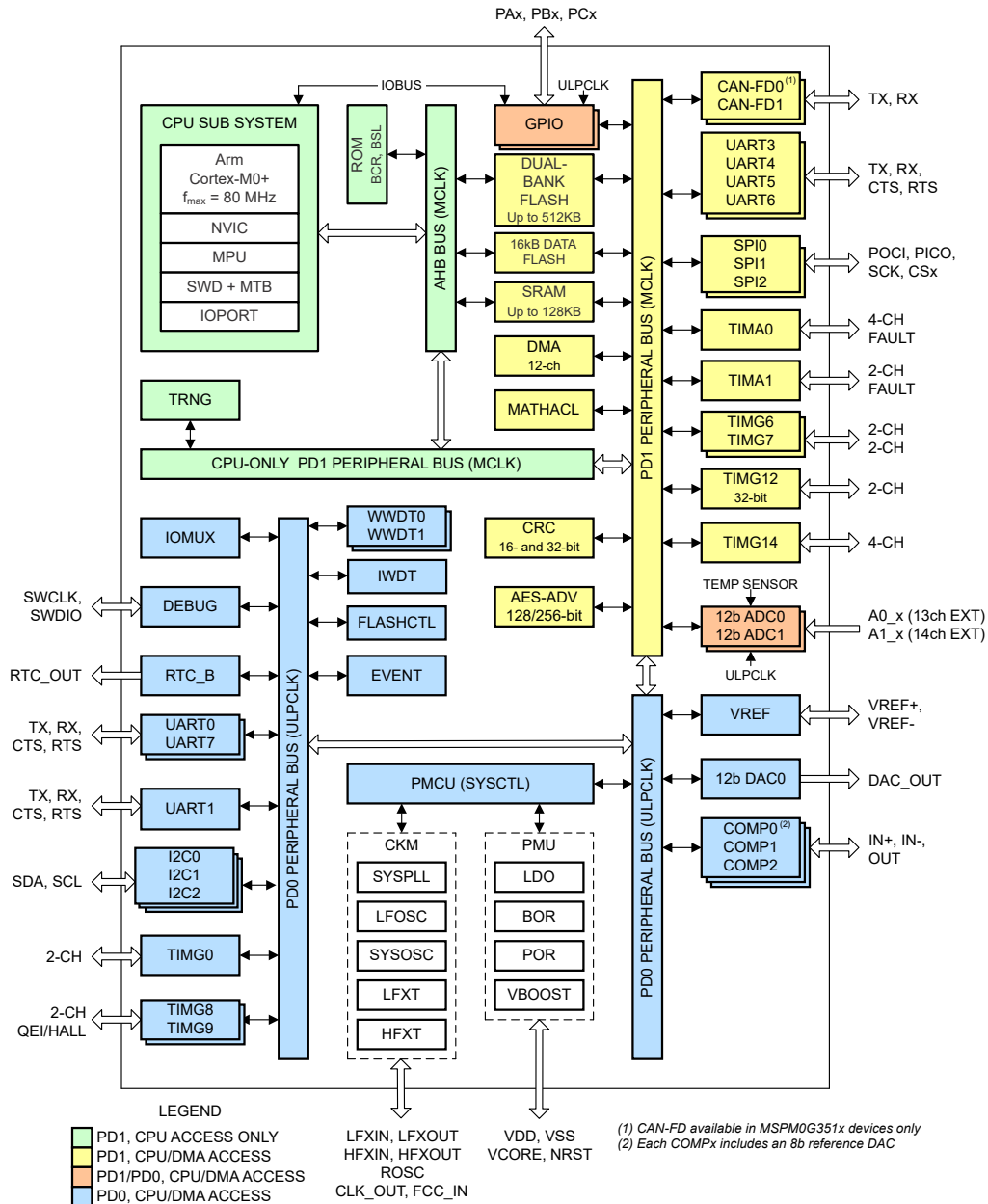
Figure 4-1. MSPM0Gx51x Block Diagram
