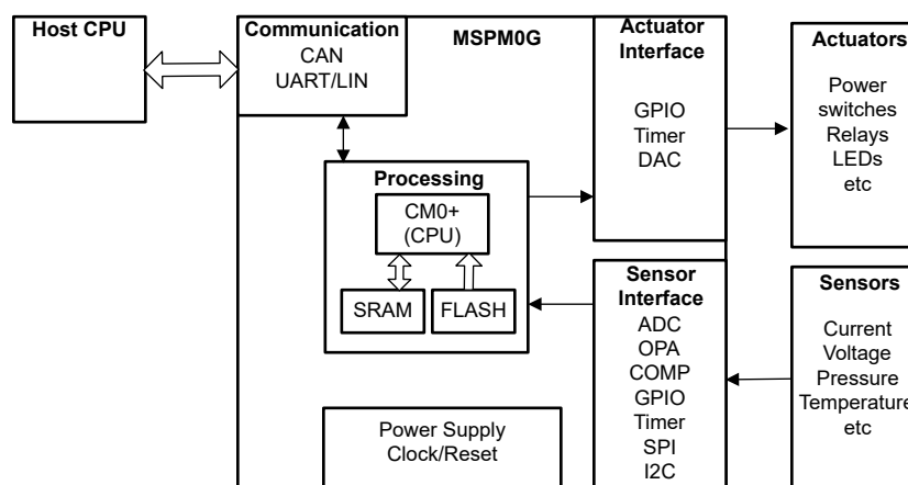
Figure 4-2. MSPM0Gx51x Typical Application
