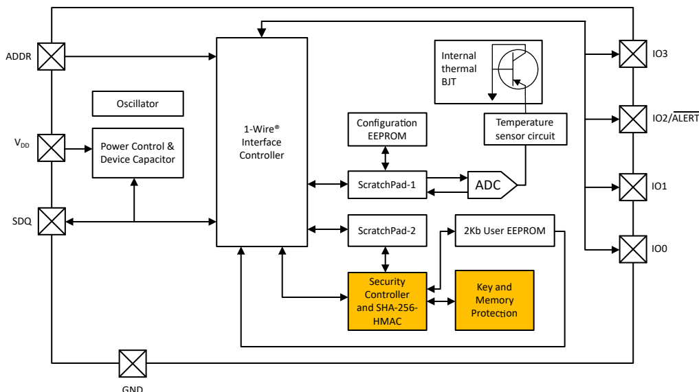
Figure 1-1. Functional Block Diagram with 1-Wire® controller
