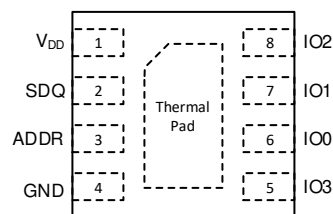
Figure 4-1. Pin Diagram (WSON-8 Package)
