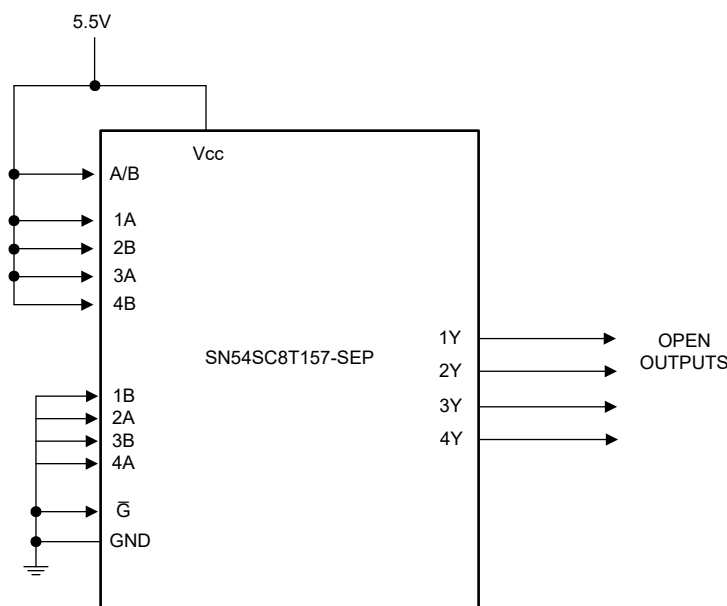
Figure 2-1. SN54SC8T157-SEP Bias Diagram
