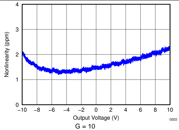
Figure 38. Gain Nonlinearity
