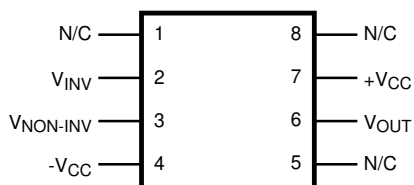
図 4-1. NAB Package, 8-Pin CDIP (Top View)
