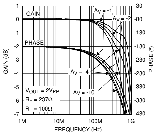
FIG 5-3. Inverting Frequency Response
