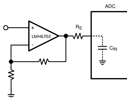
Figure 6-4. Input Amplifier to ADC
