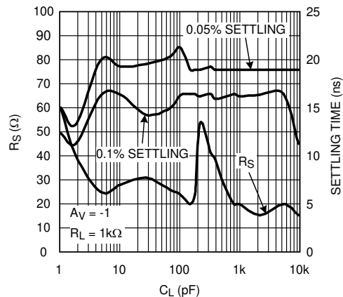
図 5-10. R_S and Settling Time vs C_L
