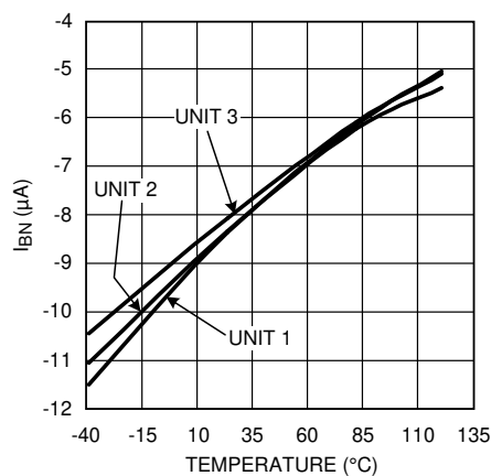
FIG 5-13. Noninverting Input Bias for Three Representative Units
