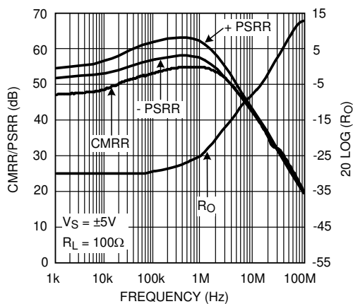
FIG 5-15. CMRR, PSRR, R_{OUT}
