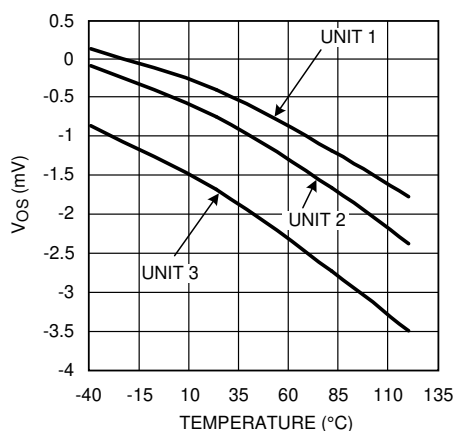
図 5-11. Input Offset for Three Representative Units
