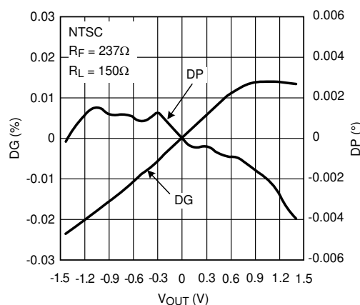
FIG 5-17. DG/DP (NTSC)
