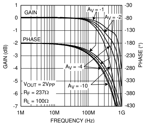
FIG 5-1. Inverting Frequency Response
