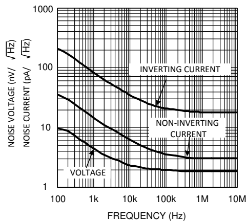
FIG 5-14. Noise
