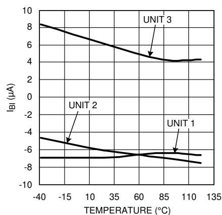
図 5-12. Inverting Input Bias for Three Representative Units
