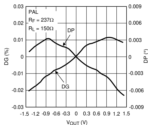
FIG 5-18. DG/DP (PAL)
