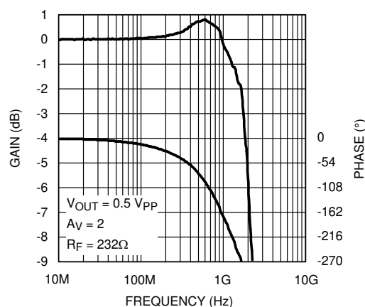
FIG 5-4. Small-Signal Bandwidth
