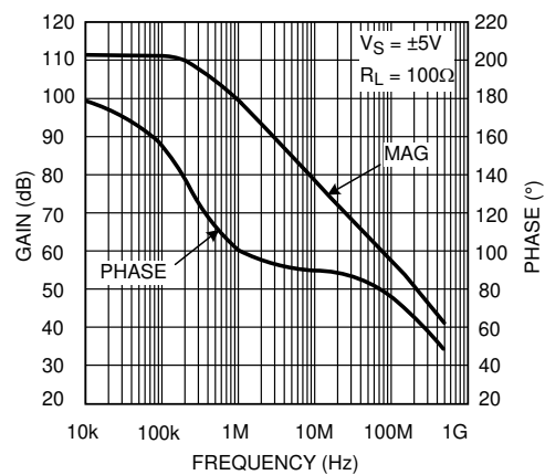
FIG 5-16. Transimpedance
