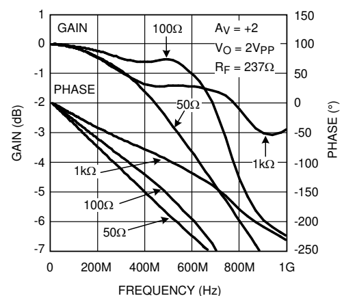
FIG 5-5. Frequency Response for Various R_L , A_V = +2
