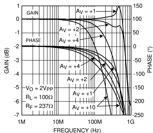
FIG 5-2. Noninverting Frequency Response
