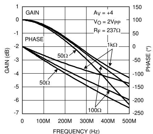
FIG 5-6. Frequency Response for Various R_L , A_V = +4
