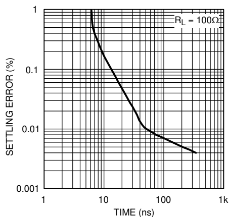
図 5-9. Percent Settling vs Time
