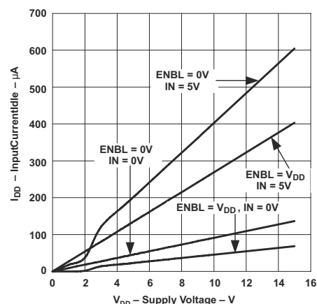
図 7-4. Input Current Idle vs Supply Voltage (UCC27322-Q1)
