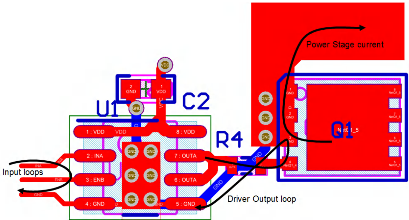
図 11-1. Layout Recommendation
