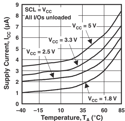
FIG 6-2. Standby Supply Current vs Temperature
