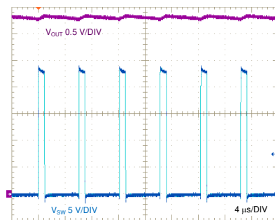
Figure 8-28. SW Node and Output Ripple Voltages, Full Load
