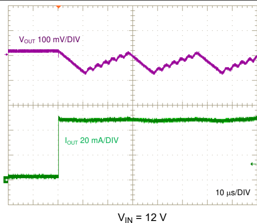
Figure 8-19. Load Transient, 0 mA to 50 mA, 1 A/ \mu\text{s}
