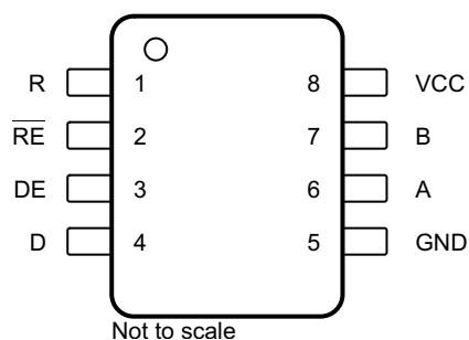
7-1. D or P Package, 8-Pin SOIC or PDIP (Top View)
