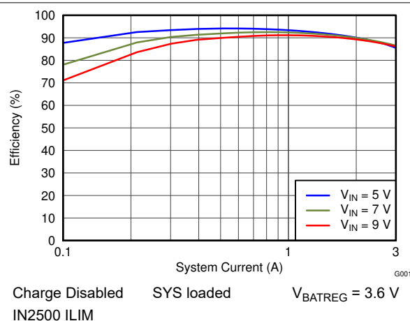
FIG 7-1. IN Efficiency
