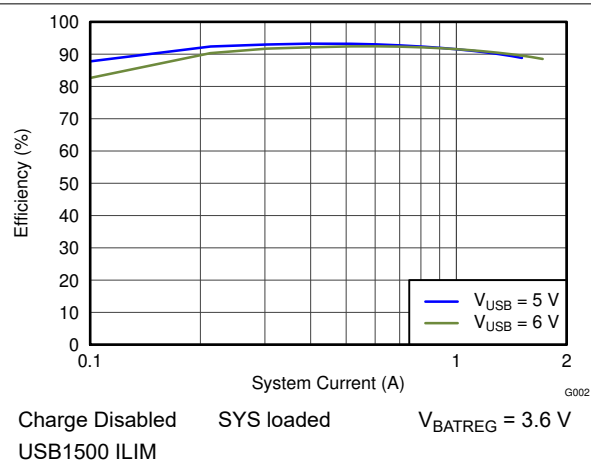
FIG 7-2. USB Efficiency
