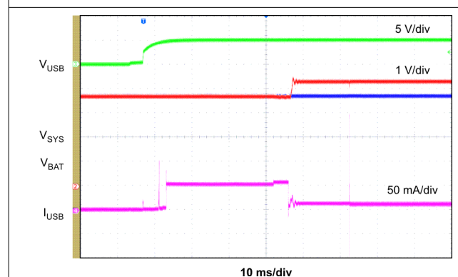
☒ 9-5. Adapter Detection USB
