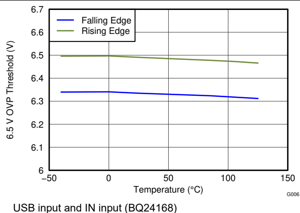
FIG 7-6. 6.5-V OVP Threshold vs Temperature
