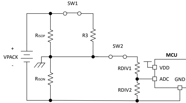
FIG 9-5. Battery V- Reference Switch Positions for ADC2 Measurement
