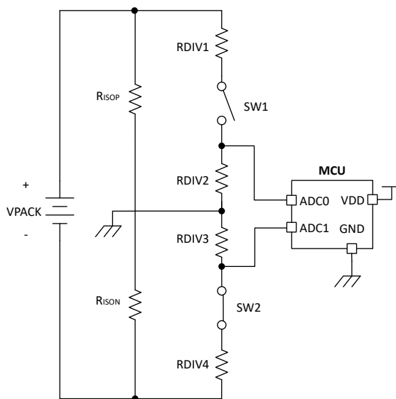
9-7. Chassis Ground Reference Switch Positions for ADC2 Measurement
