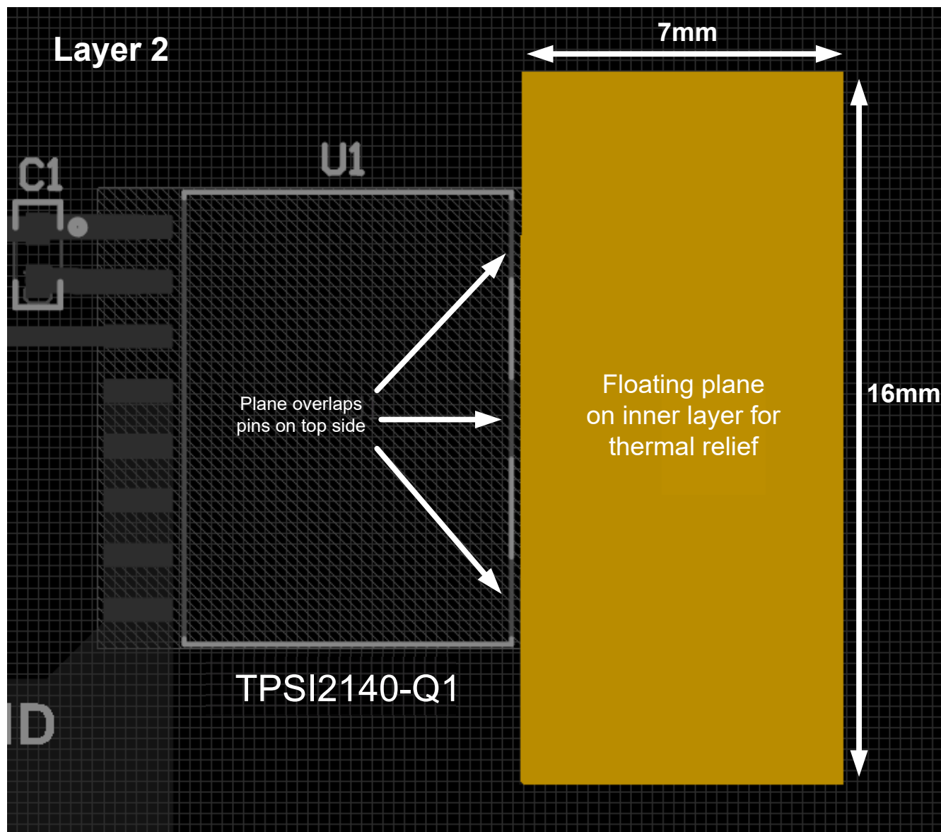
9-18. TPSI2140-Q1 Secondary Side Layout Recommendation for Optimized Thermal Performance: Inner Layer 2
