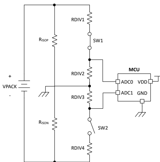
9-6. Chassis Ground Reference Switch Positions for ADC1 Measurement
