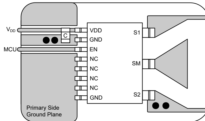
Figure 9-21. TPSI2140-Q1 Layout with Interlayer Stitch Capacitance: Top Layer (1)
