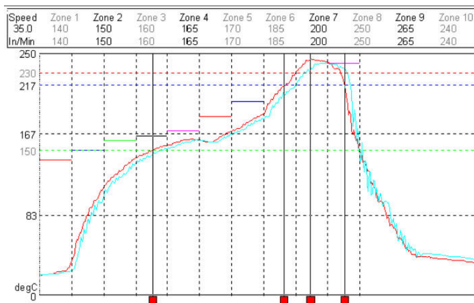
9-16. Recommended Solder Reflow Temperature Profile
