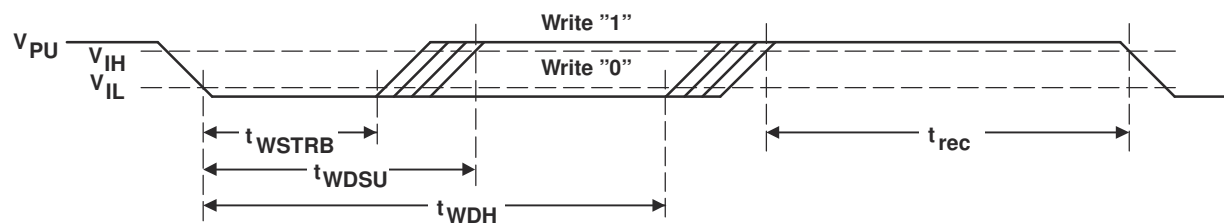
FIG 7-10. WRITE Bit Timing Diagram
