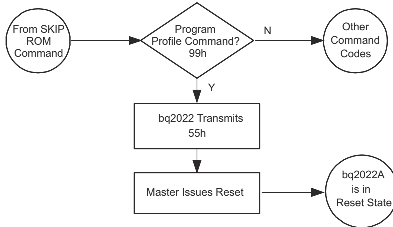
FIG 7-8. PROGRAM PROFILE Command Flow
