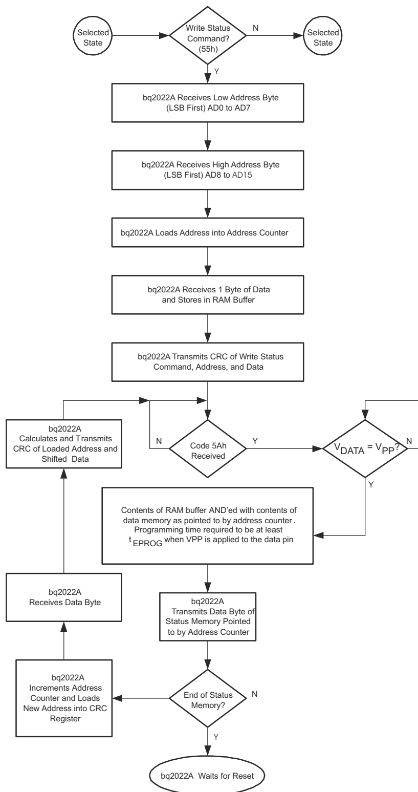
7-7. WRITE STATUS Command Flow
