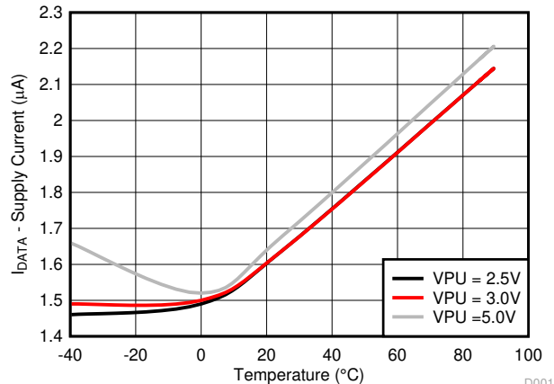
FIG 8-3. Supply Current vs. Temperature
