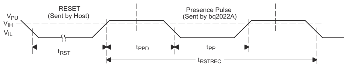
FIG 7-9. Reset Timing Diagram
