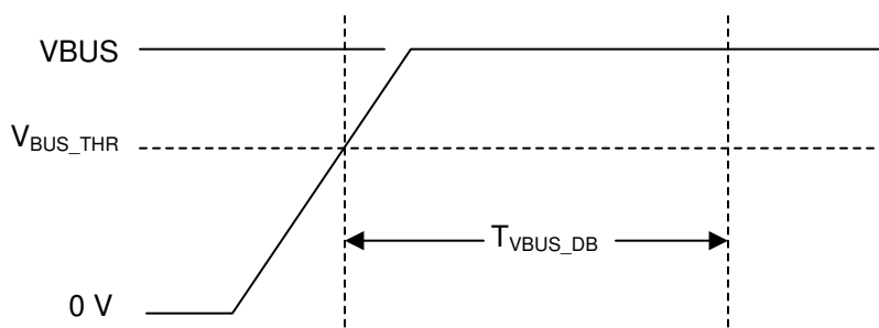
6-1. VBUS Detect and Debounce
