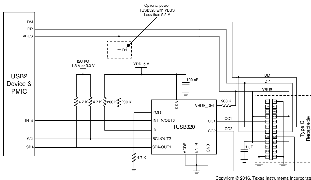
❏ 8-11. UFP in I 2 C Mode Schematic
