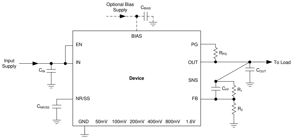
图 8-4. Adjustable Operation
