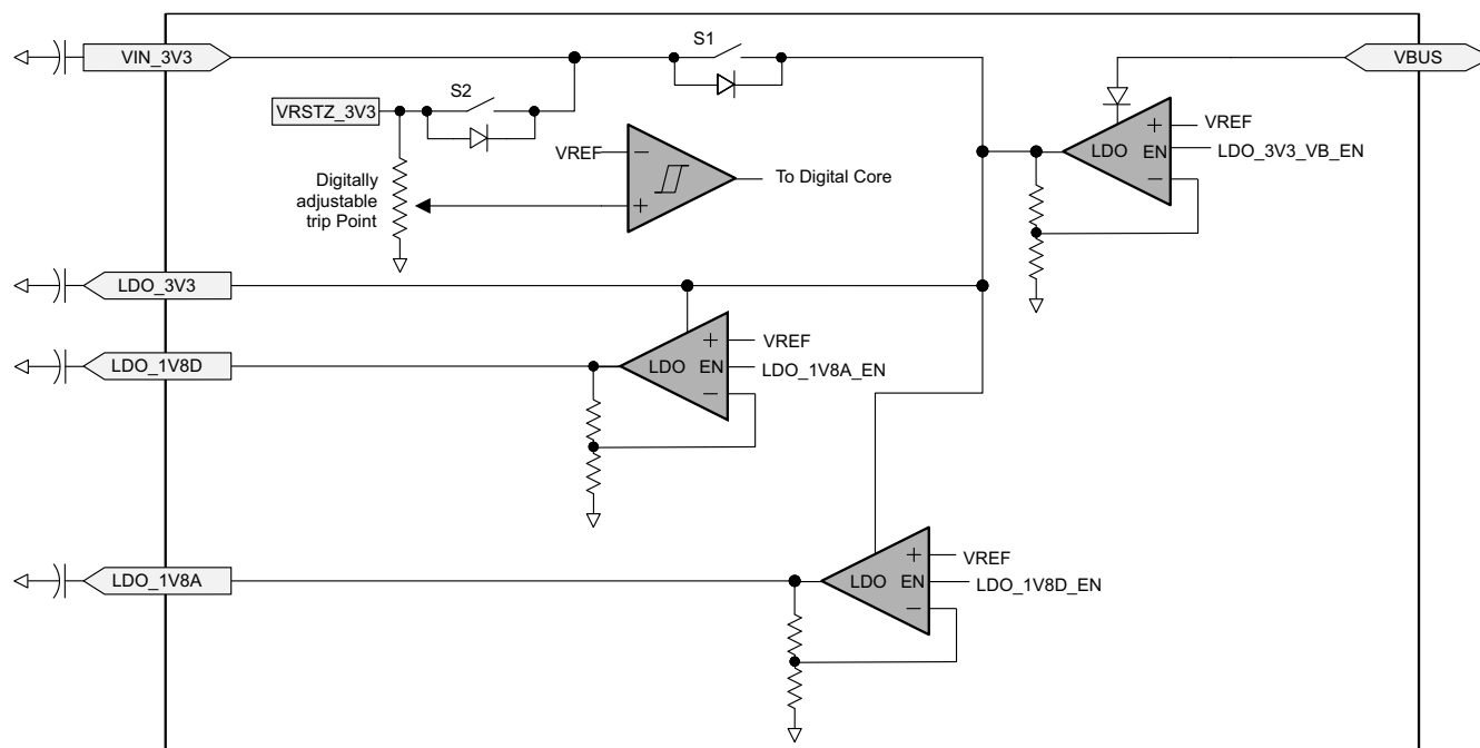
9-40. Power Supply Path
