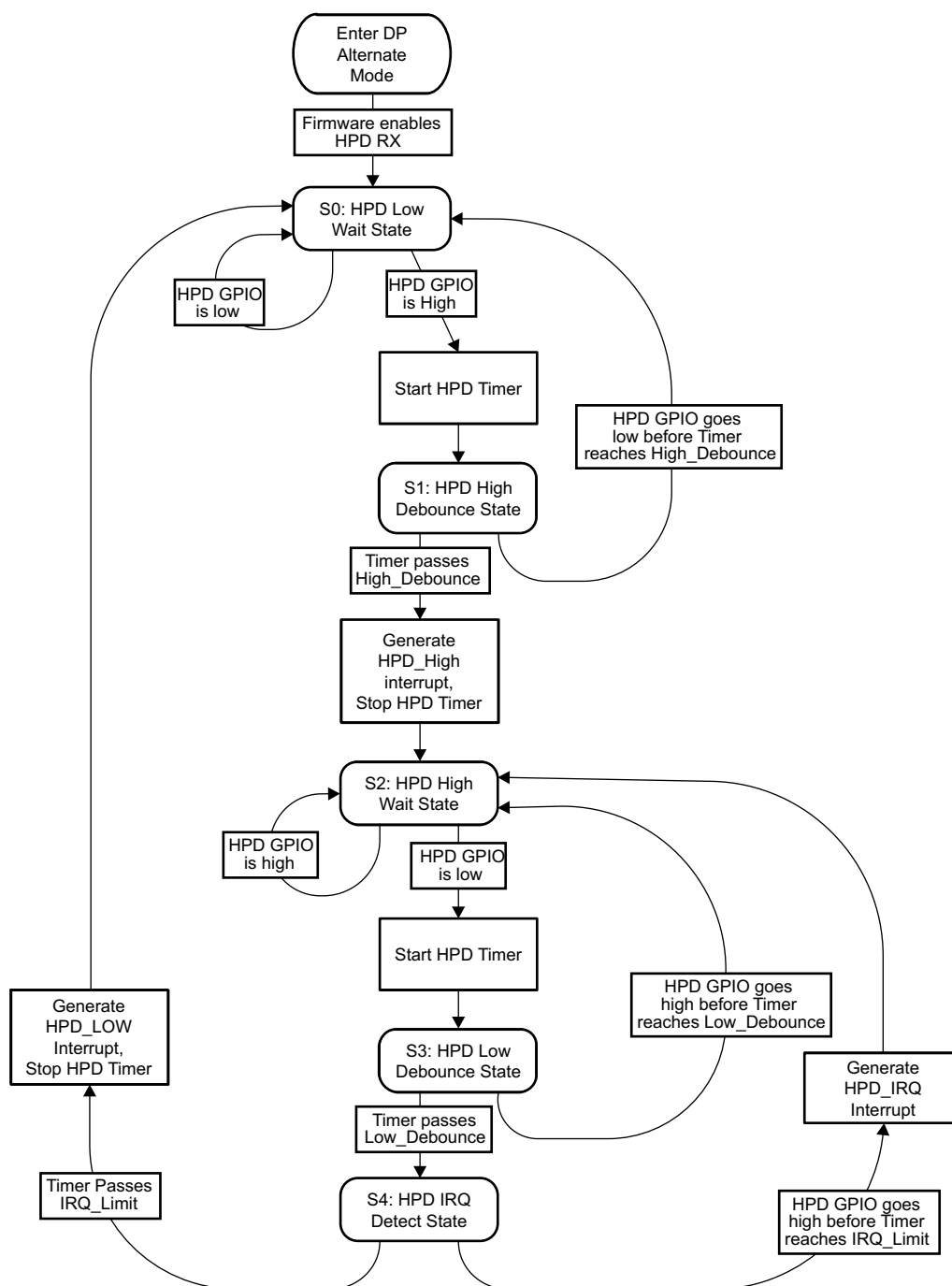
9-42. HPD RX Flow
