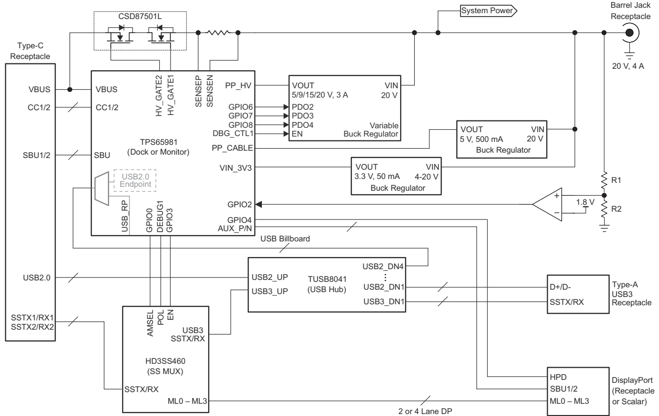
图 10-3. Type-C and PD Dock or Monitor Application
