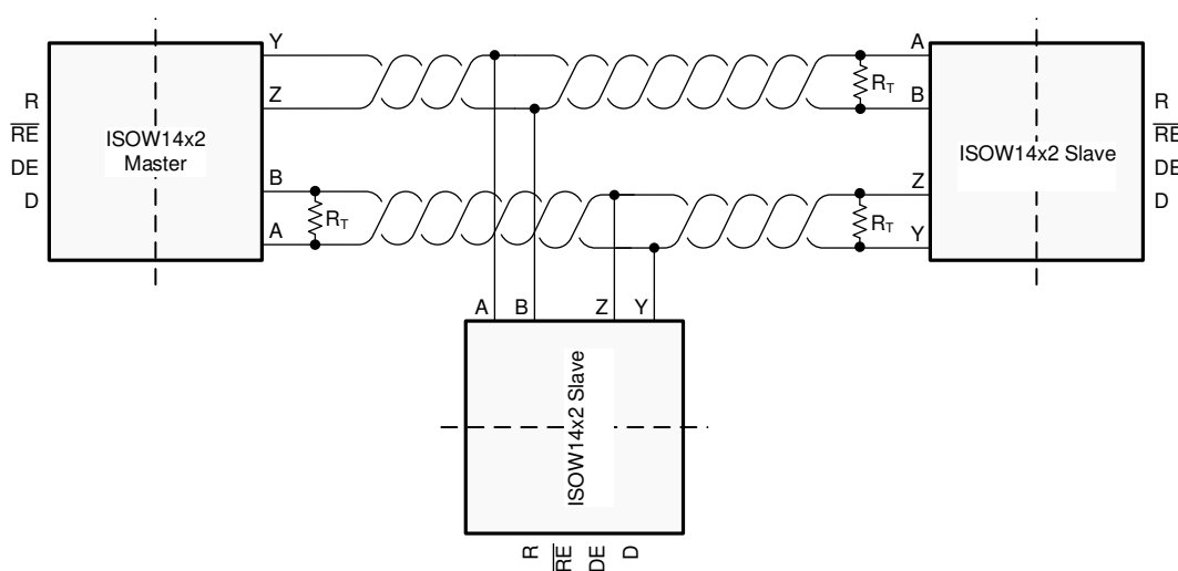
☒ 11-1. Typical RS-485 network with Full-duplex Isolated transceivers
