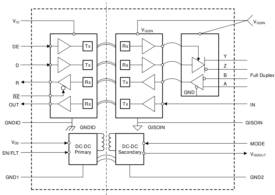
10-1. Block Diagram
