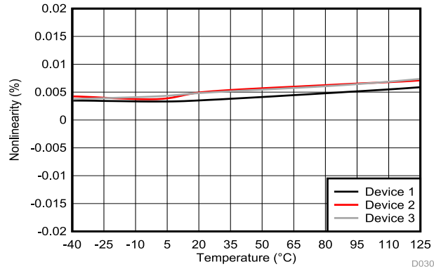
FIG 6-17. Nonlinearity vs Temperature
