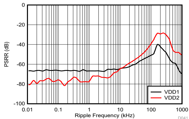
FIG 6-30. Power-Supply Rejection Ratio vs Ripple Frequency
