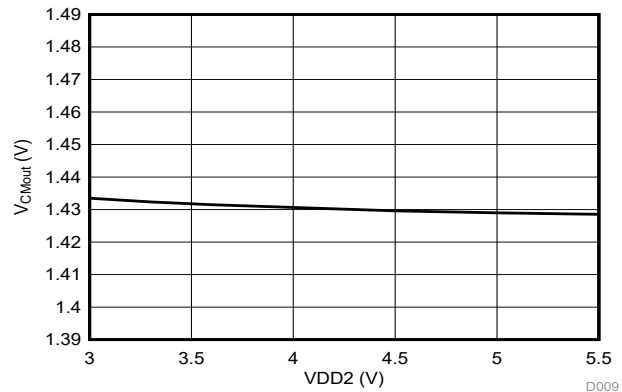
FIG 6-32. Common-Mode Output Voltage vs Supply Voltage
