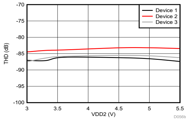
Figure 6-19. Total Harmonic Distortion vs Input Voltage
