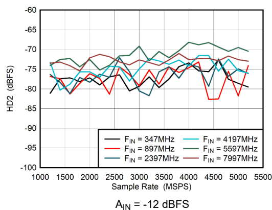
5-52. Dual Channel Mode: HD2 vs Sample Rate
