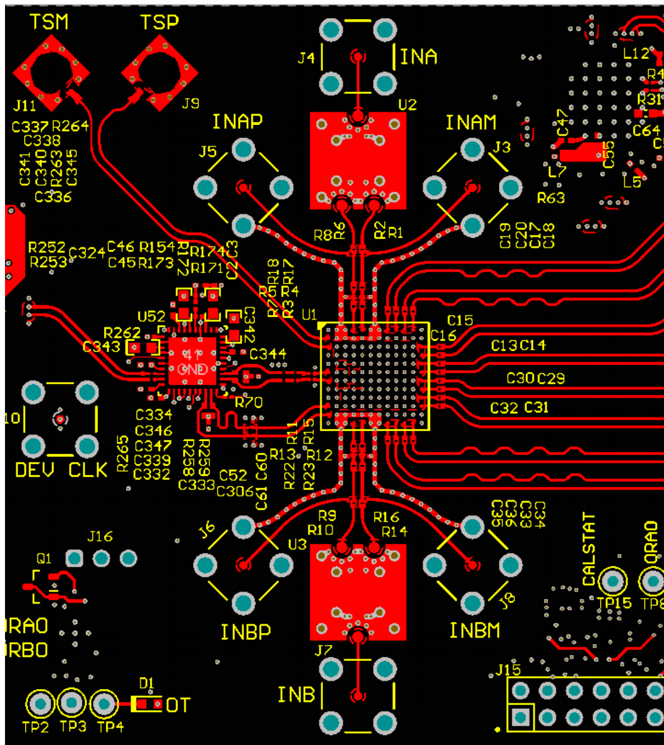
7-4. Top Layer Routing: Analog Inputs, CLK and SYSREF, DA0-3, DB0-3
