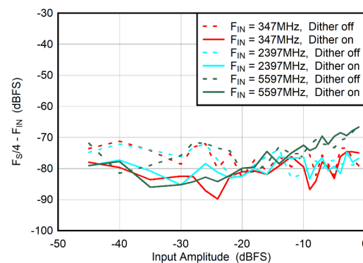
図 5-70. DES Mode: F_S/4 - F_{\text{IN}} vs Input Amplitude and Dither
