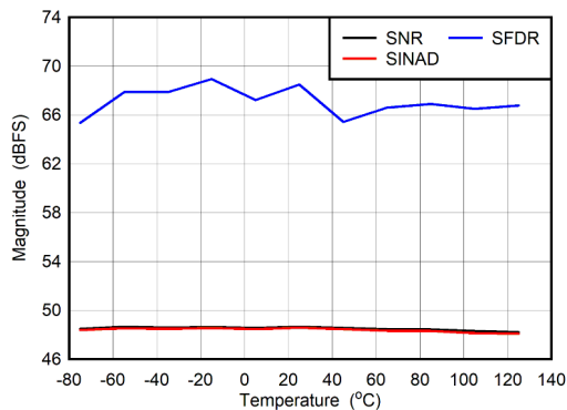
FIG 5-89. Dual Channel Mode: SNR, SINAD and SFDR vs Temperature
