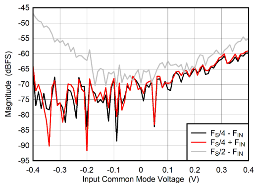
FIG 5-99. DES Mode: F_S/2 - F_{\text{IN}} , F_S/4 \pm F_{\text{IN}} vs Input Common Mode Voltage
