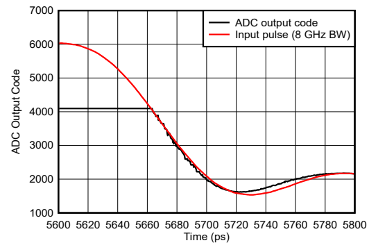
FIG 5-124. Pulse Overdrive Recovery Zoomed
