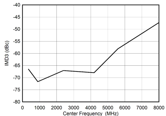
FIG 5-100. DES Mode: IMD3 vs Input Frequency
