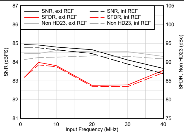
6-27. AC Performance vs Input Frequency
