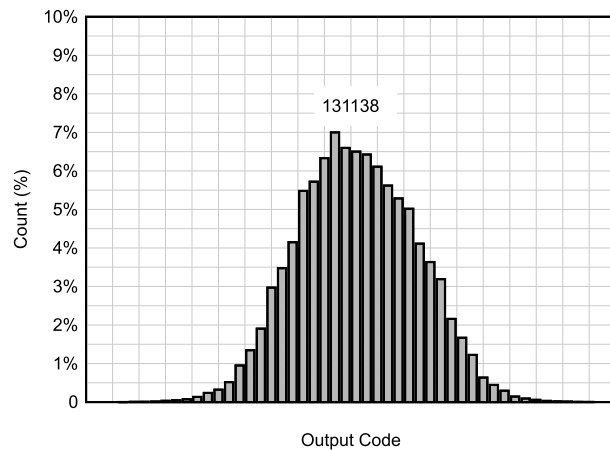
FIG 6-62. DC Offset Histogram
