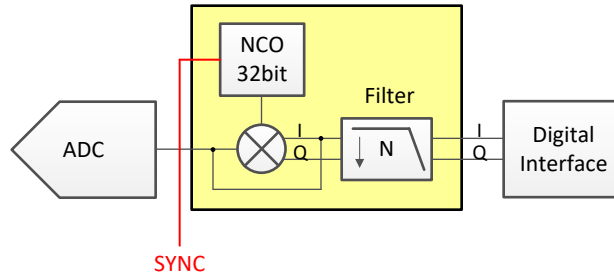
8-21. Internal Digital Decimation Filter
