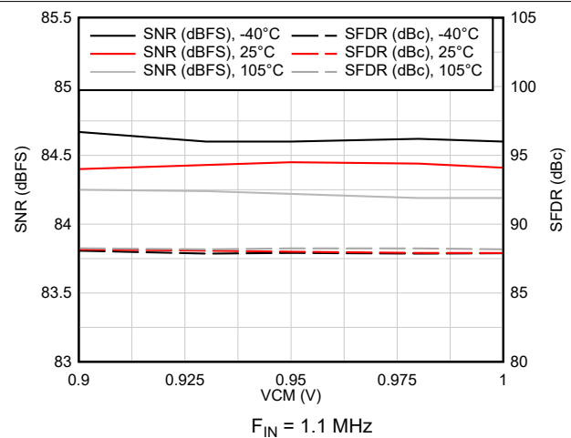
FIG 6-33. AC Performance vs VCM vs Temperature
