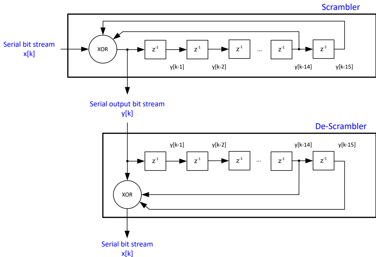
Figure 8-42. Output scrambler and descrambler operation
