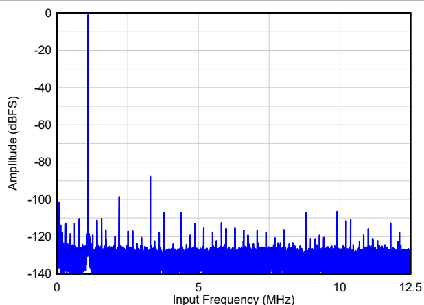
FIG 6-18. Single Tone FFT at F_{IN} = 1.1 MHz
