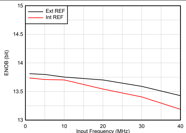
FIG 6-6. ENOB vs Input Frequency
