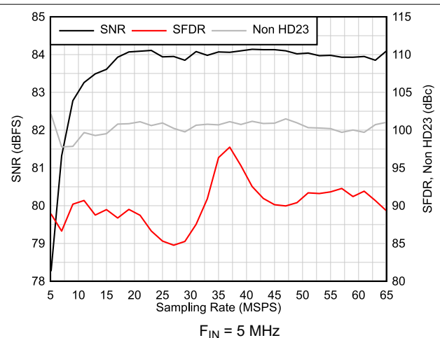
FIG 6-53. AC Performance vs Sampling Rate
