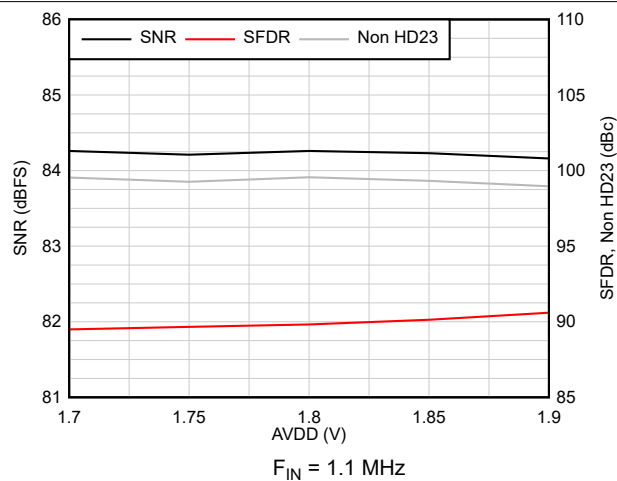
FIG 6-32. AC Performance vs AVDD
