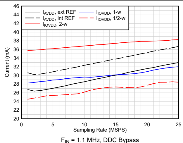
FIG 6-37. Current vs Sampling Rate
