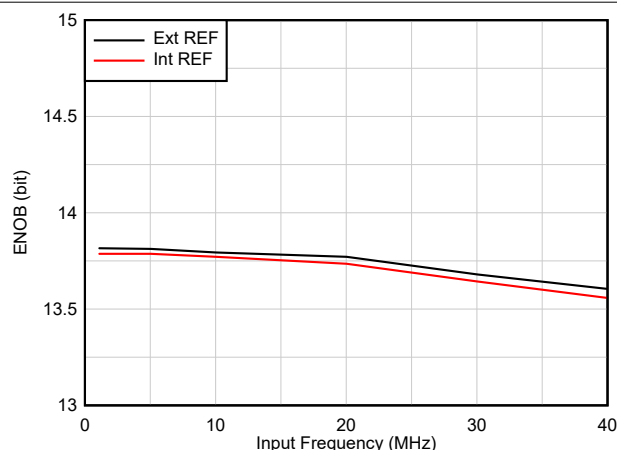
6-28. ENOB vs Input Frequency
