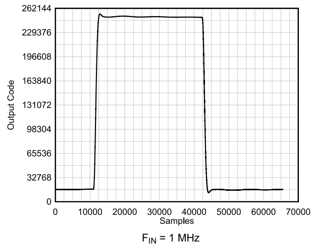
FIG 6-63. Pulse Response
