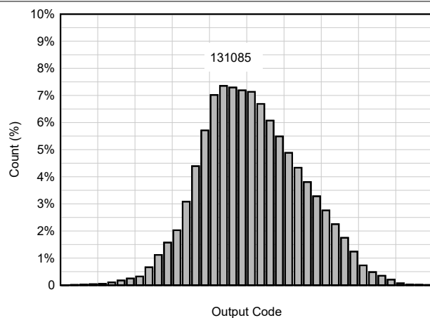
FIG 6-36. DC Offset Histogram
