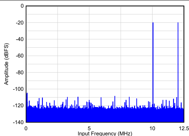
A_{IN} = -20 dBFS/tone, IMD3 = 88 dBc 6-26. Two Tone FFT at F_{IN} = 10/12 MHz
