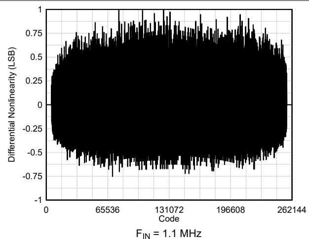
FIG 6-35. DNL vs Code
