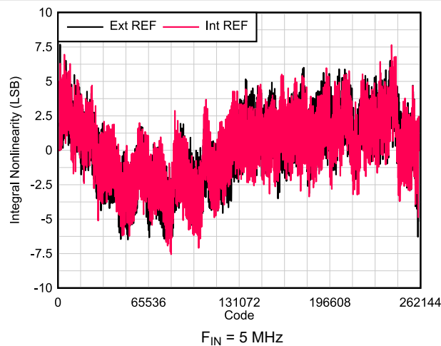
FIG 6-60. INL vs Code
