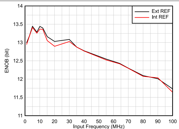
FIG 6-51. ENOB vs Input Frequency
