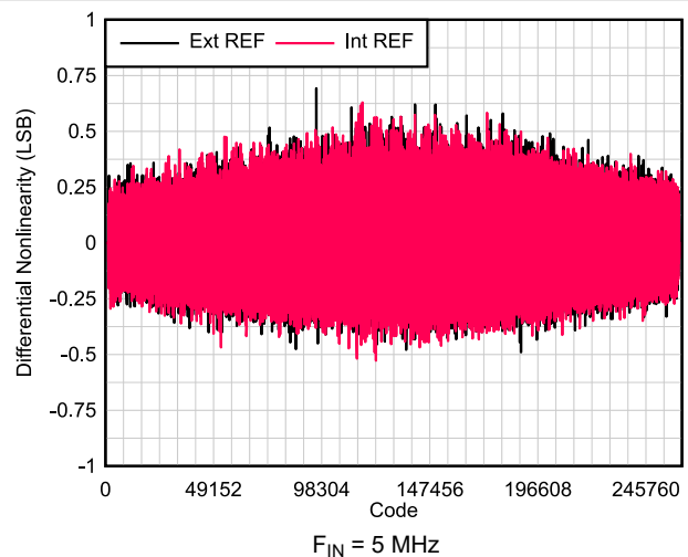
FIG 6-61. DNL vs Code
