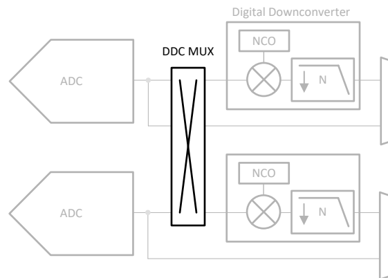
8-22. DDC MUX
