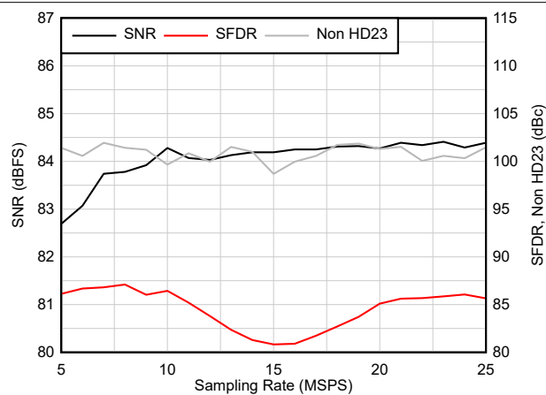
F_{IN} = 1.1 MHz 6-30. AC Performance vs Sampling Rate
