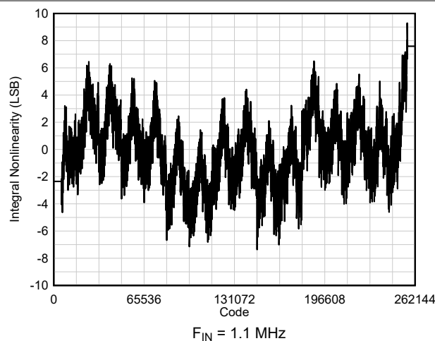
FIG 6-34. INL vs Code
