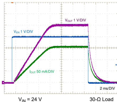
8-9. Enable ON and OFF
