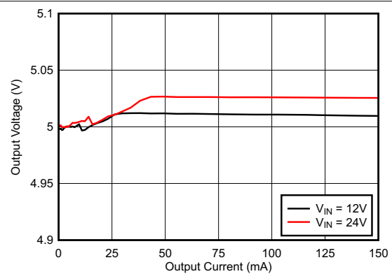
8-3. Load Regulation
