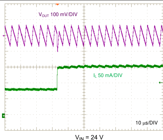
8-12. Load Transient, 50 mA to 150 mA, 1 A/ \mu s
