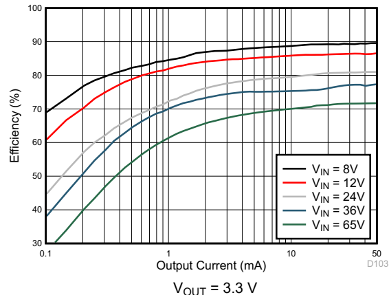
FIG 8-15. Efficiency
