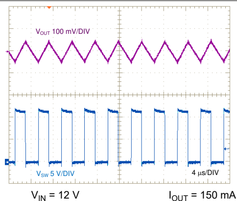
8-6. SW Node and Output Ripple Voltage, Full Load
