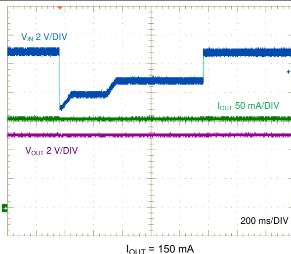
8-13. Input Transient (Automotive Cold Crank Profile)
