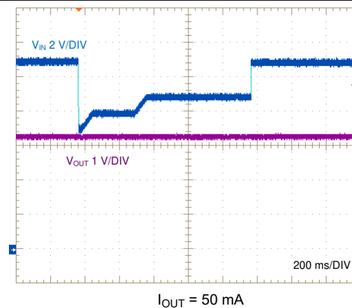
FIG 8-20. Input Voltage Transient (Automotive Cold Crank Profile)
