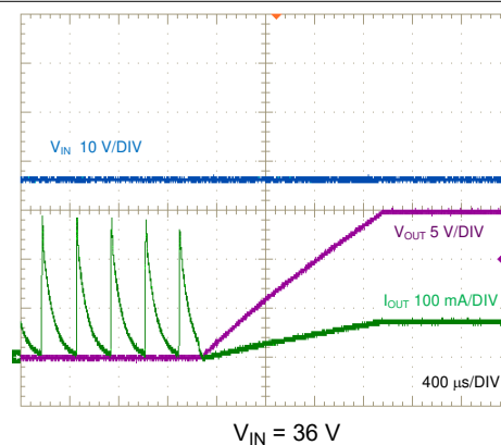
8-35. Short Circuit Recovery
