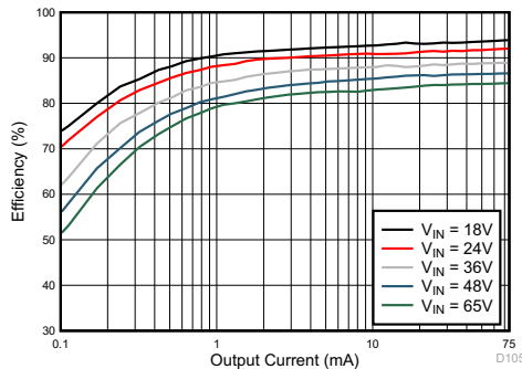
See schematic, L_F = 47\text{ }\mu\text{H} F_{SW(nom)} = 500\text{ kHz} Figure 8-21 C_{OUT} = 10\text{ }\mu\text{F} R_{ILIM} = 24.9\text{ k}\Omega
