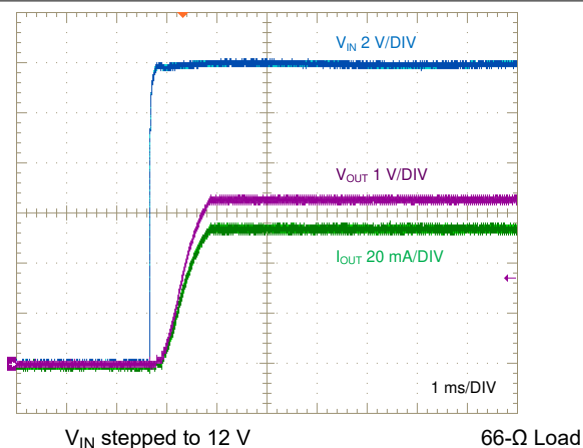
FIG 8-17. Start-Up, Full Load
