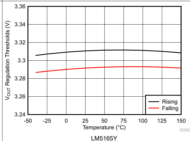
6-12. VOUT Regulation Thresholds vs Temperature
