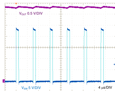
Figure 8-28. SW Node and Output Ripple Voltages, Full Load
