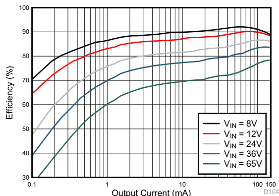
Figure 8-27. Efficiency
