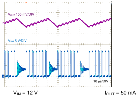
FIG 8-16. SW Node and Output Ripple Voltage, Full Load
