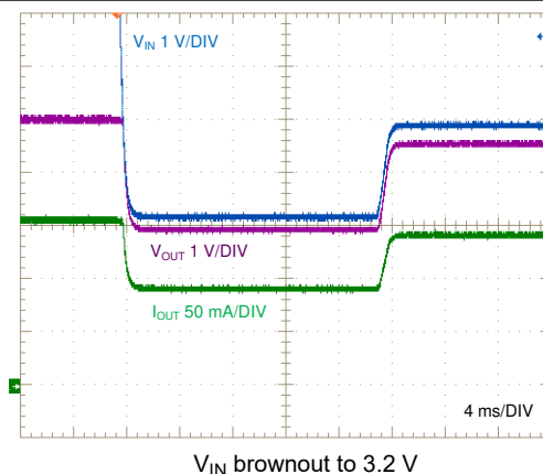
8-11. Dropout Performance, 150-mA Resistive Load
