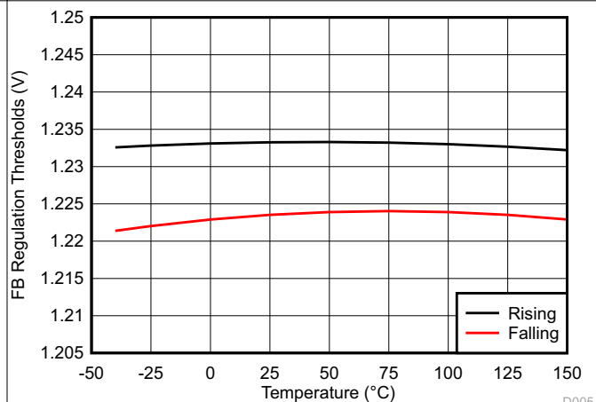
6-10. Feedback Comparator Voltage vs Temperature
