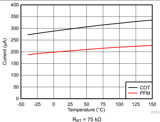
6-21. VIN Active Mode Supply Current vs Temperature
