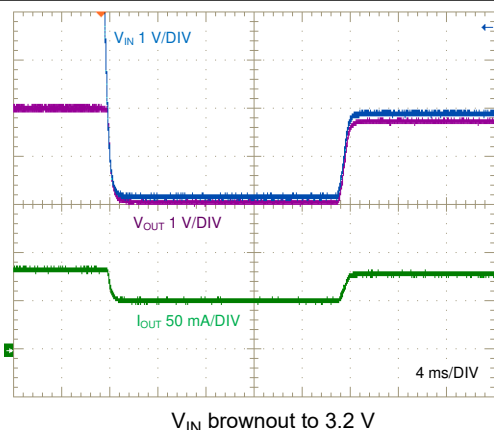
8-10. Dropout Performance, 75-mA Resistive Load
