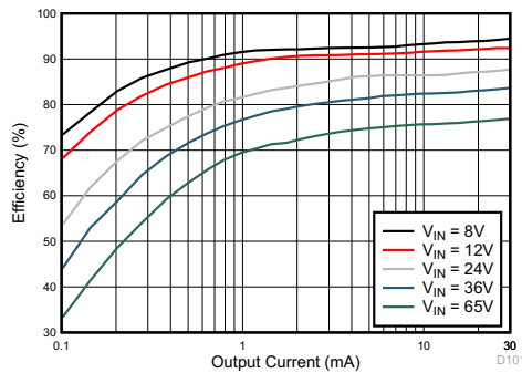
5-V, 25-mA Design L_F = 470\text{ }\mu\text{H} F_{SW(nom)} = 100\text{ kHz} C_{OUT} = 47\text{ }\mu\text{F} R_{ILIM} \geq 100\text{ k}\Omega
