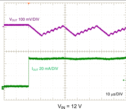
FIG 8-19. Load Transient, 0 mA to 50 mA, 1 A/μs
