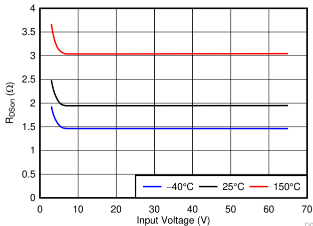
6-7. High-Side MOSFET On-State Resistance vs Input Voltage
