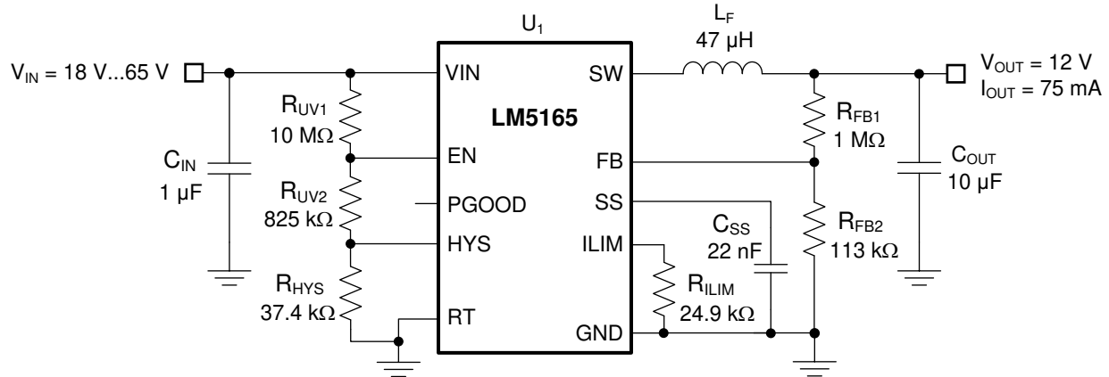
8-21. Schematic for Design 3 With V_{IN(nom)} = 24\text{ V} , V_{OUT} = 12\text{ V} , I_{OUT(max)} = 75\text{ mA} , F_{SW(nom)} = 500\text{ kHz}
