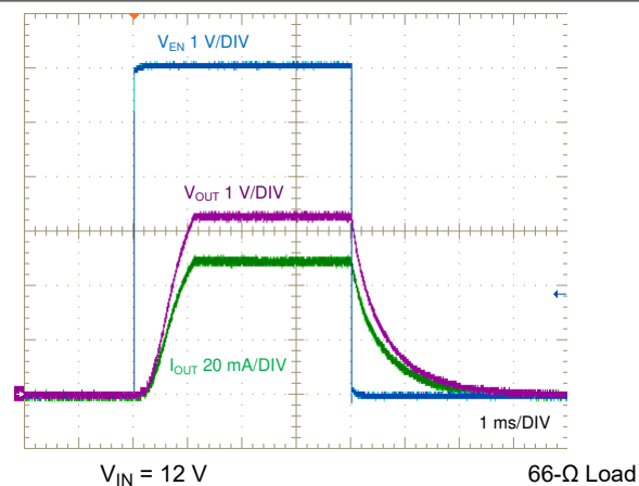
FIG 8-18. Enable ON and OFF
