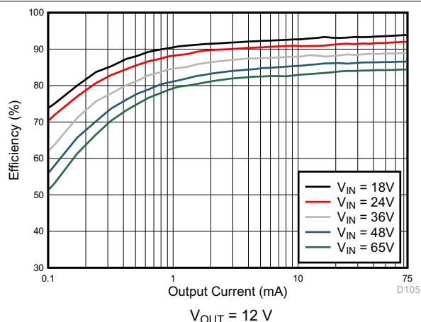
8-22. Efficiency
