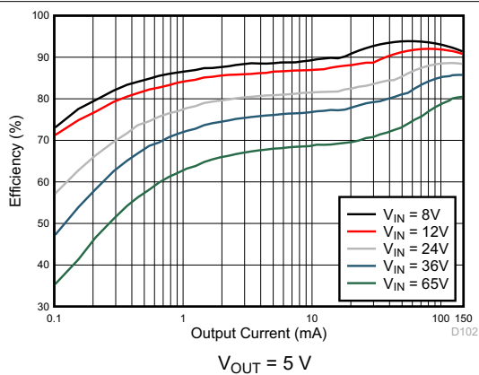
8-2. Efficiency
