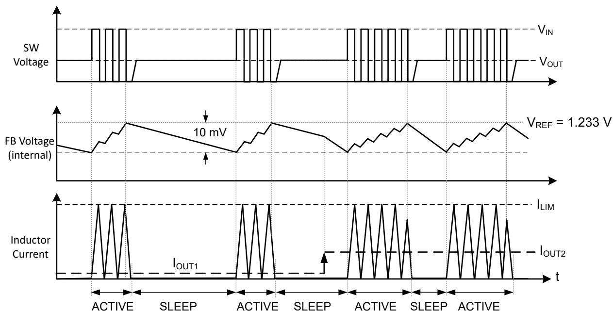
FIG 7-3. PFM Mode SW Node Voltage, Feedback Voltage, and Inductor Current Waveforms
