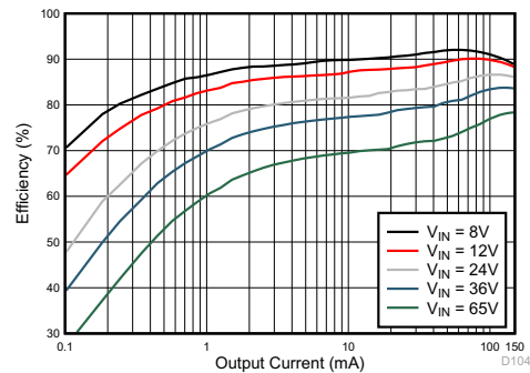
See schematic, L_F = 150\text{ }\mu\text{H} F_{SW(nom)} = 160\text{ kHz} Figure 8-26 C_{OUT} = 22\text{ }\mu\text{F} R_{RT} = 121\text{ k}\Omega
