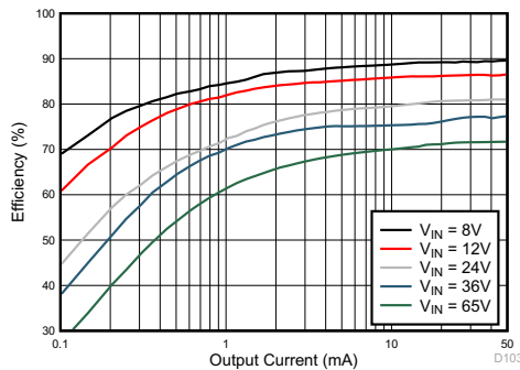
See schematic, L_F = 47\text{ }\mu\text{H} F_{SW(nom)} = 350\text{ kHz} Figure 8-14 C_{OUT} = 10\text{ }\mu\text{F} R_{ILIM} = 56.2\text{ k}\Omega
