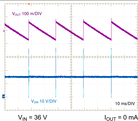
8-33. SW Node and Output Ripple Voltage, No Load
