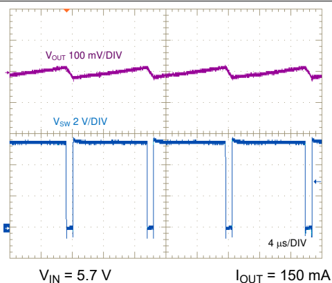
8-7. SW Node and Output Ripple Voltage Showing Frequency Foldback Near Dropout
