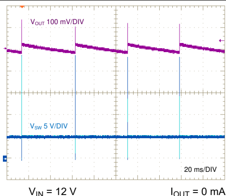
8-5. SW Node and Output Ripple Voltage, No Load
