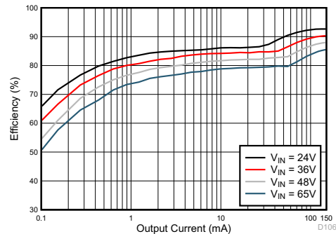
See schematic, L_F = 150\text{ }\mu\text{H} F_{SW(nom)} = 600\text{ kHz} Figure 8-29 C_{OUT} = 10\text{ }\mu\text{F} R_{RT} = 143\text{ k}\Omega
