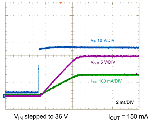
8-31. Start-Up, Full Load
