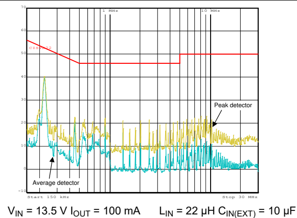
8-4. EMI Plot – CISPR 22 Filtered Emissions
