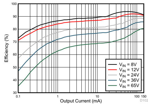
See schematic, L_F = 220\text{ }\mu\text{H} F_{SW(nom)} = 230\text{ kHz} Figure 8-1 C_{OUT} = 22\text{ }\mu\text{F} R_{RT} = 133\text{ k}\Omega
