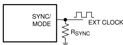
❏ 7-13. Frequency Synchronization
