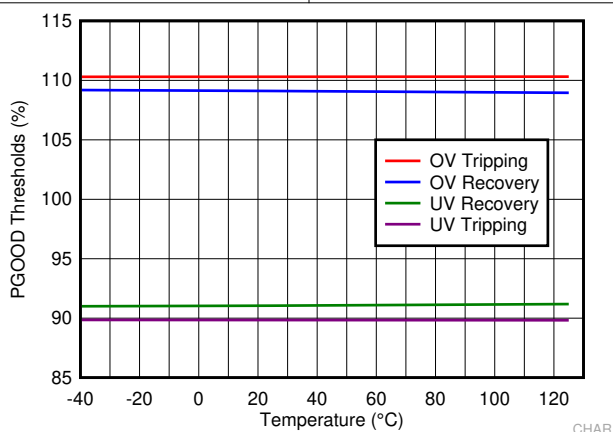
FIG 6-9. PGOOD Thresholds
