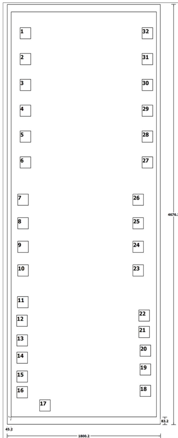
図 5-2. TPS7H4010-SEP Bare Die Diagram
