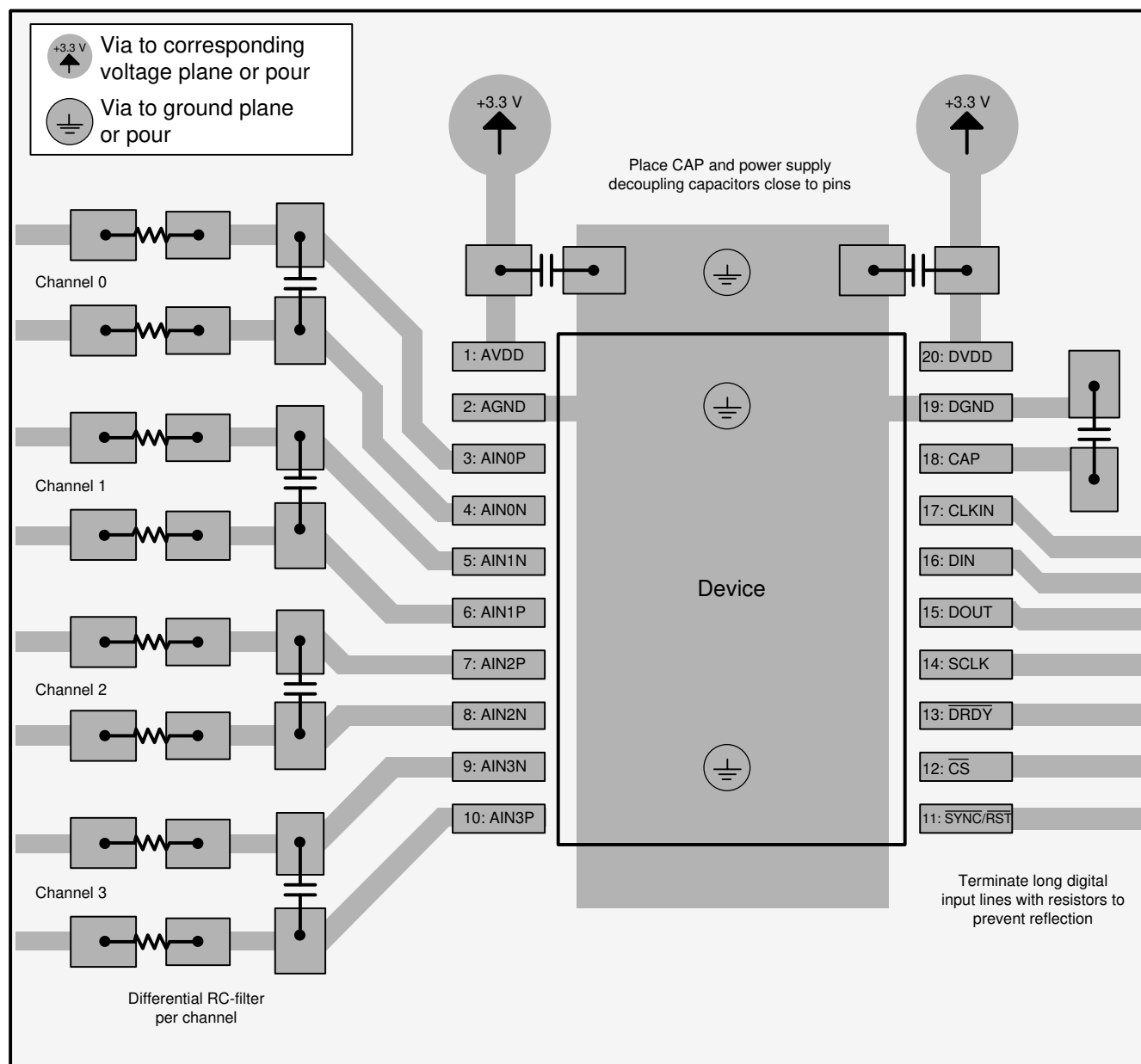
☒ 11-1. Layout Example
