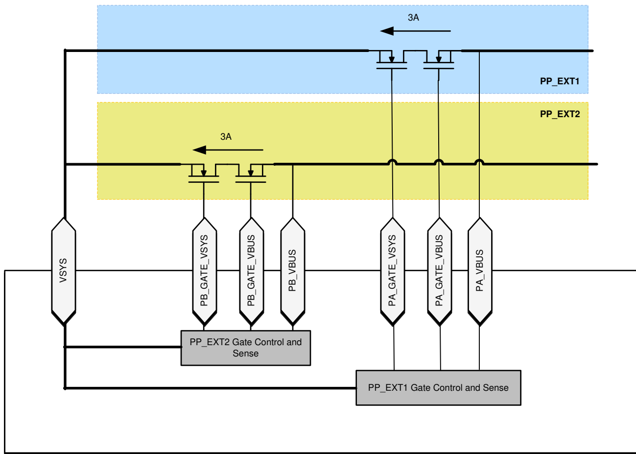
8-11. Sink Path Control
