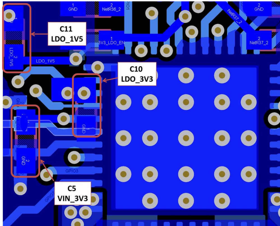
FIG 11-8. VIN_3V3, LDO_3V3, and LDO_1V5 Routing
