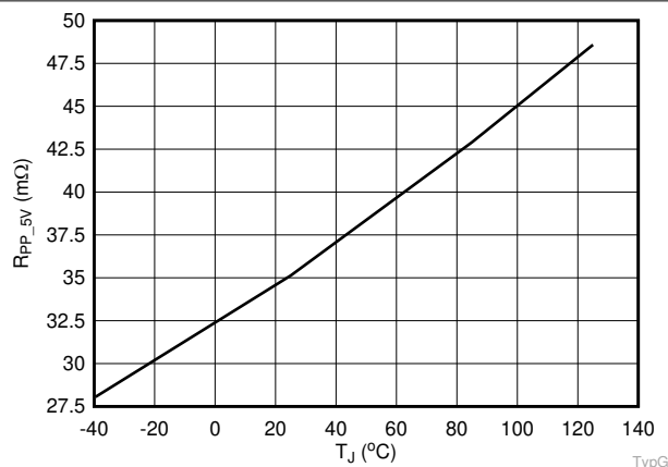
图 6-1. PP_5Vx Rdson vs. Temperature
