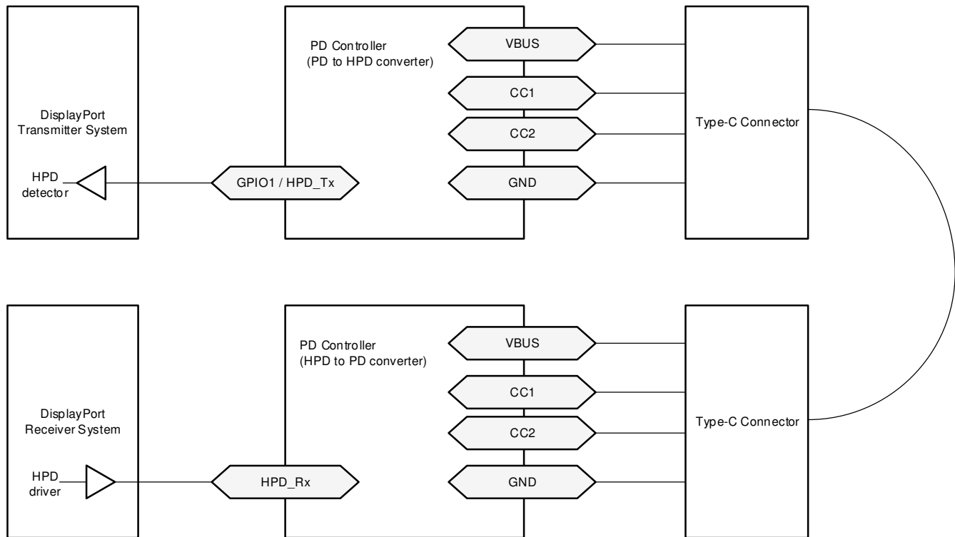
图 8-19. Illustration of how a PD-to-HPD Converter Passes the HPD Signal Along in a DisplayPort System
