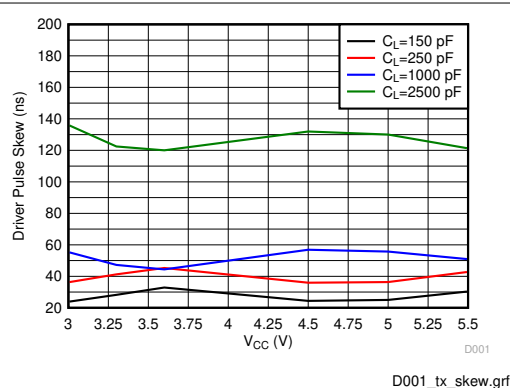
5-4. Driver Pulse Skew (RGT Package)
