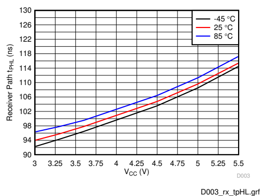
5-6. Receiver Path High-to-Low Propagation Delay (RGT Package)
