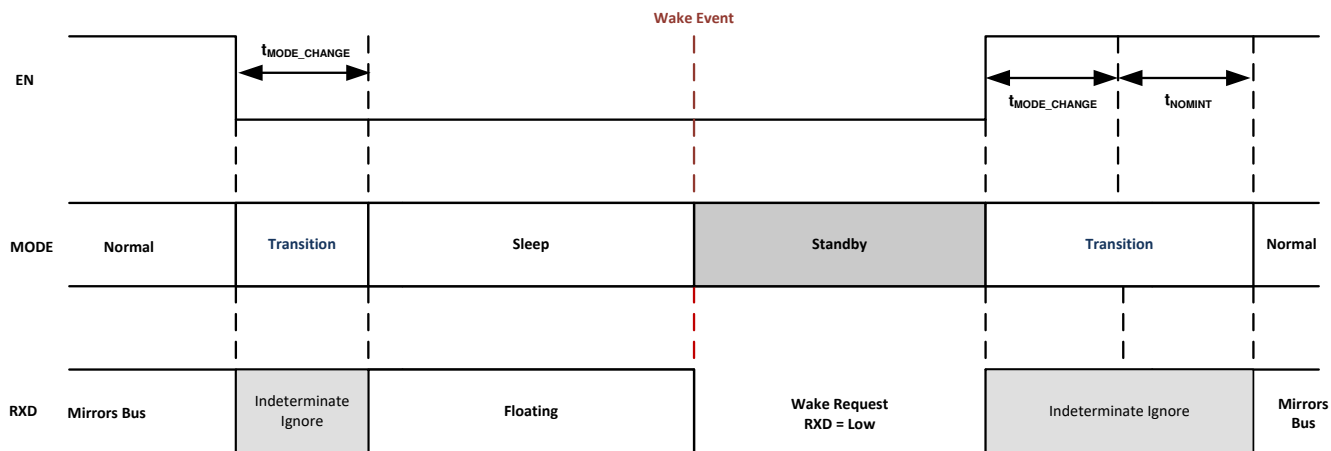
8-14. Mode Transitions
