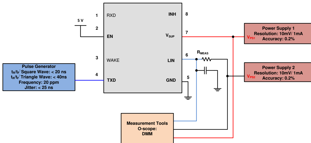
8-10. Test Circuit Slope Control and Duty Cycle Param 27, 28, 29, 30 , 72, 73, 74, 75
