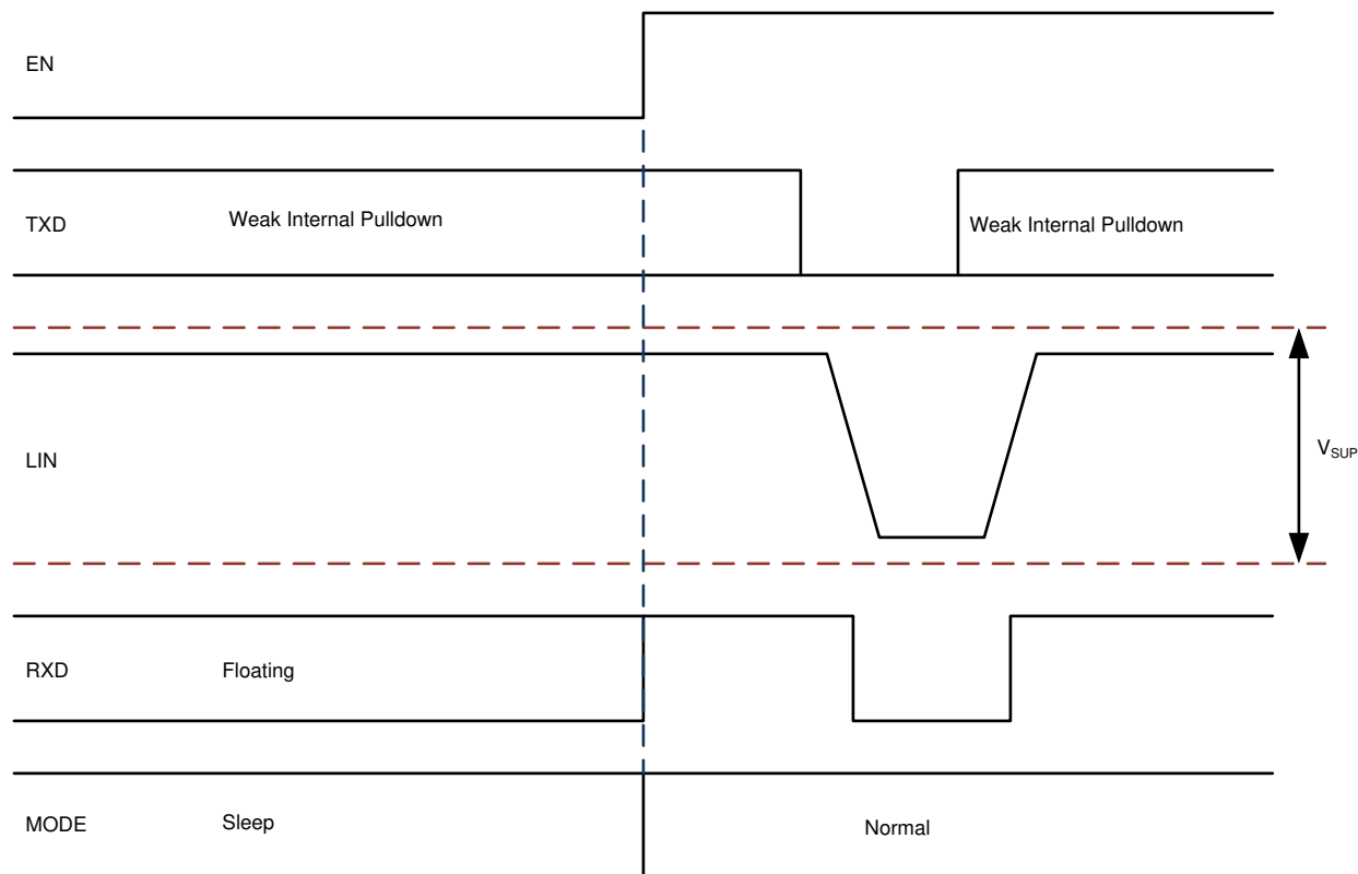
8-14. Mode Transitions
