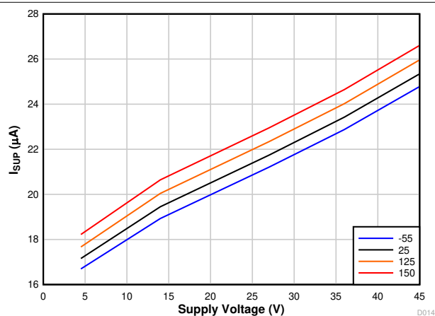
7-6. Standby Mode I_{SUP} Recessive vs V_{SUP} and Temperature
