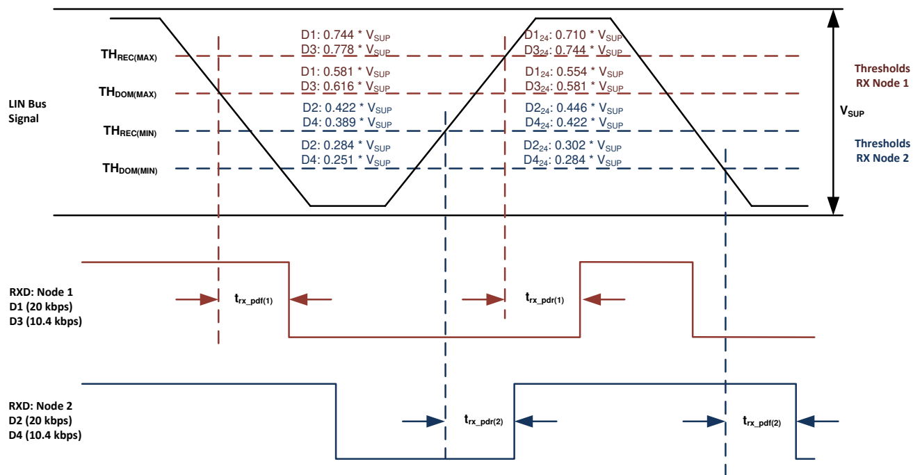
🔍 8-13. Propagation Delay
