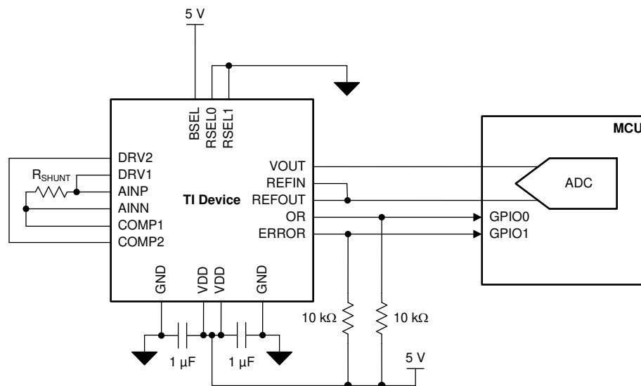
図 67. Linear-Position Sensing
