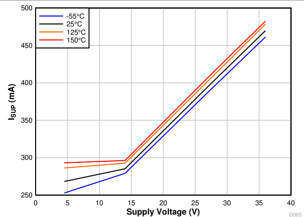
7-4. I_{SUP} Recessive vs V_{SUP} and Temperature
