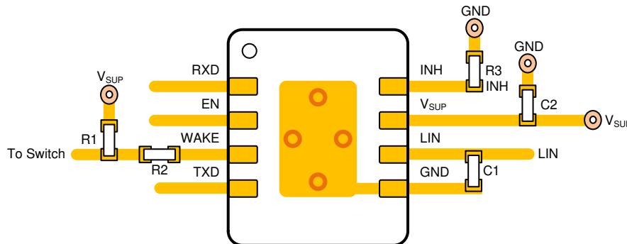
Figure 10-4. Layout Example
