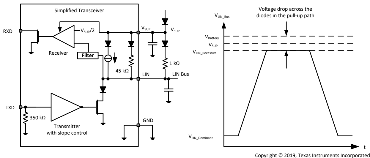
9-1. Commander Node Configuration with Voltage Levels
