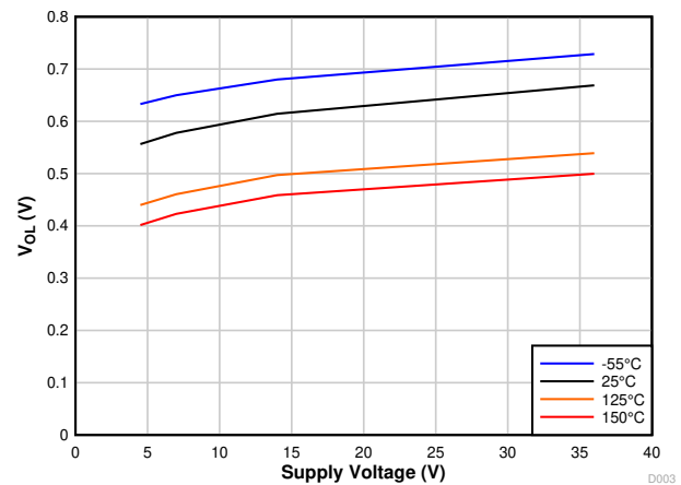
7-2. V_{OL} vs V_{SUP} and Temperature
