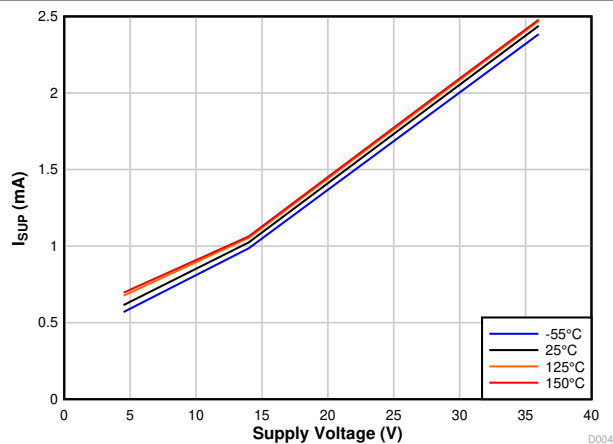
7-3. I_{SUP} Dominant vs V_{SUP} and Temperature
