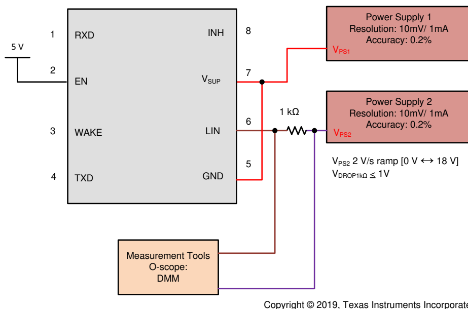
8-9. Test Circuit for I_{BUS\_NO\_GND} Loss of GND
