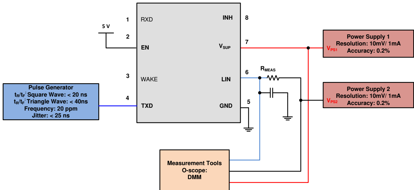
8-13. Propagation Delay Test Circuit; Param 31, 32
