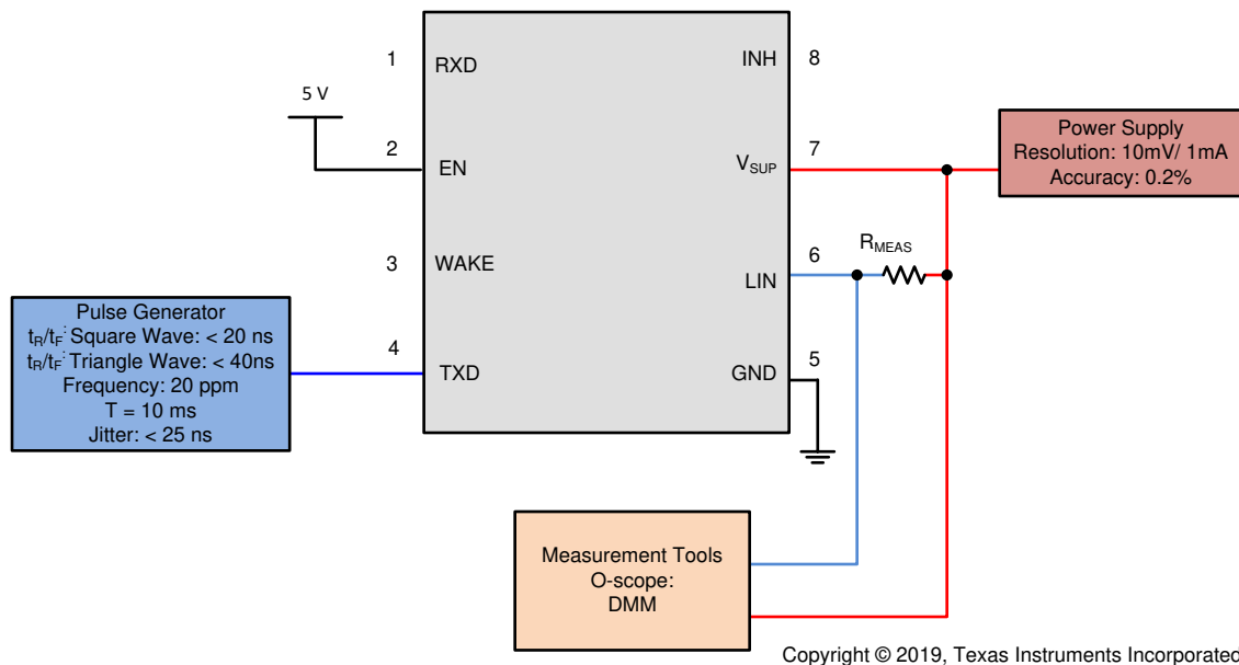
8-6. Test Circuit for I_{BUS\_LIM} at Dominant State (Driver on) Param 12
