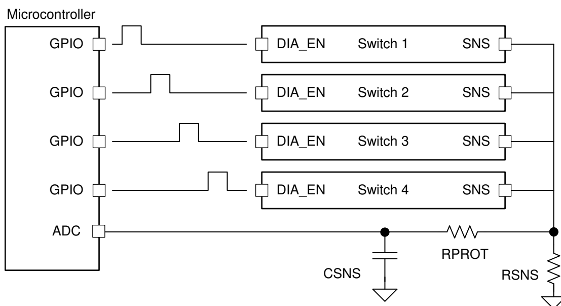
図 12. Sharing R SNS Among Multiple Devices
