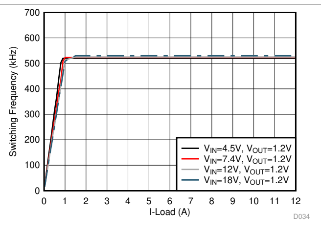
Figure 22. Switching Frequency vs Output Load
