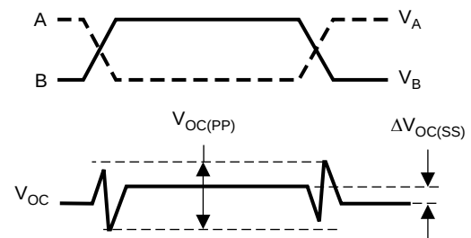
Figure 10. Measurement of Driver Differential Output Voltage With Common-Mode Load
