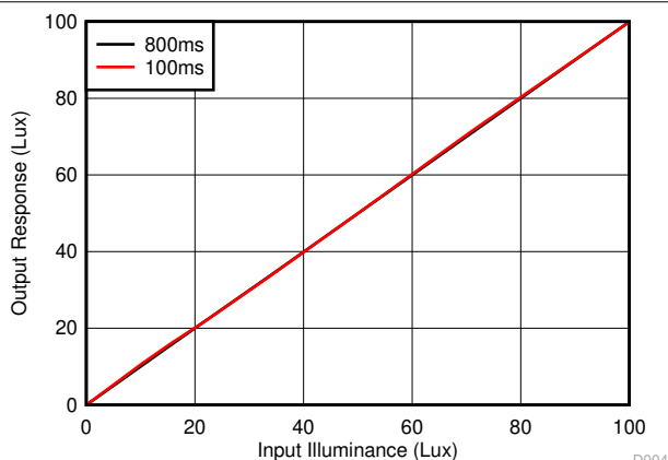
7-6. Output Response vs Input Illuminance (Mid Range = 0 lux to 100 lux)
