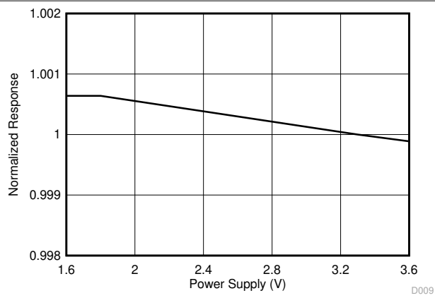
7-13. Normalized Response vs Power-Supply Voltage
