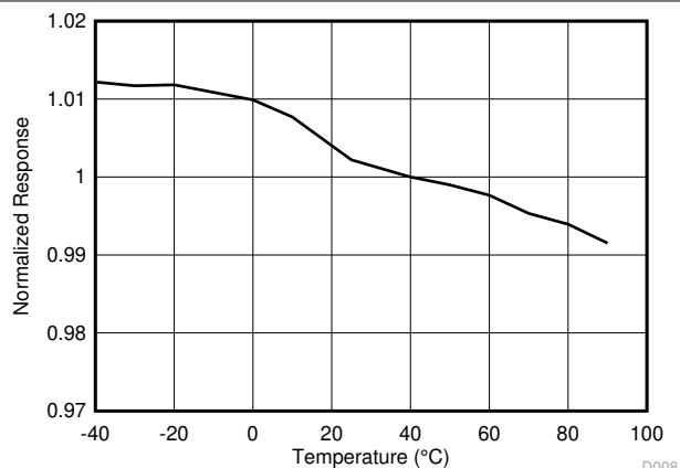
7-11. Normalized Response vs Temperature
