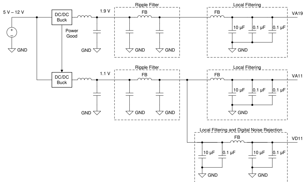
FIG 9-2. DC/DC Switching Regulator Example
