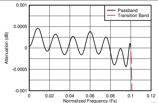
Figure 7-12. Decimate-by-4 Composite Zoomed Pass-Band Response (D4_AP87 = 0)
