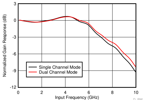
FIG 6-68. Gain Response vs Input Frequency
