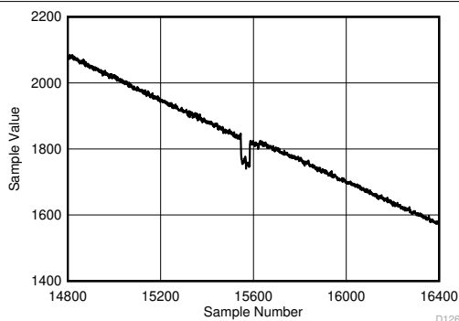
FIG 6-70. Background Calibration Core Transition (AC Signal Zoomed)
