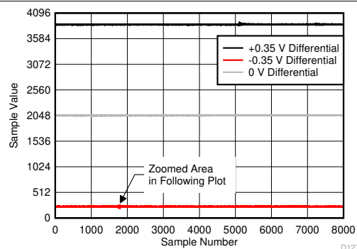
FIG 6-71. Background Calibration Core Transition (DC Signal)
