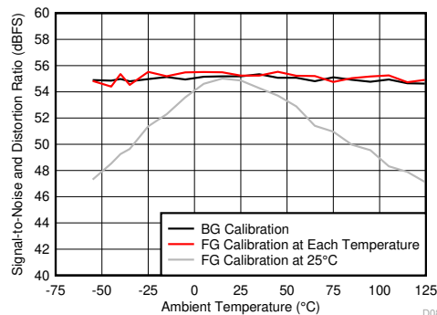
FIG 6-52. SINAD vs Temperature and Calibration Mode
