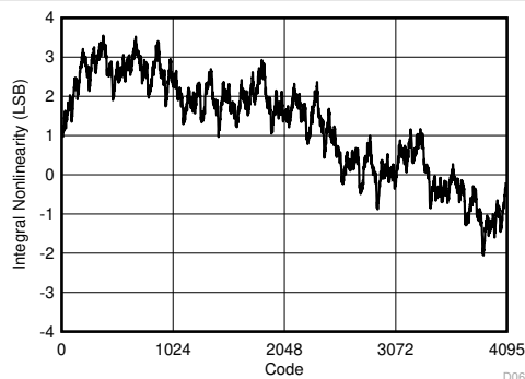
JMODE 1, FG calibration, f_s = 6400\text{ MSPS} , f_{\text{IN}} = 99.97\text{ MHz}
