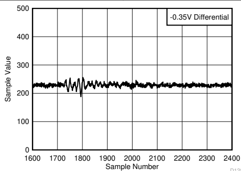
FIG 6-70. Background Calibration Core Transition (AC Signal Zoomed)
