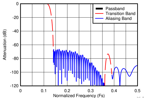
Figure 7-13. Decimate-by-4 Composite Response (D4_AP87 = 1)
