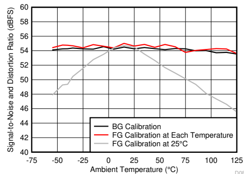
FIG 6-53. SINAD vs Temperature and Calibration Mode
