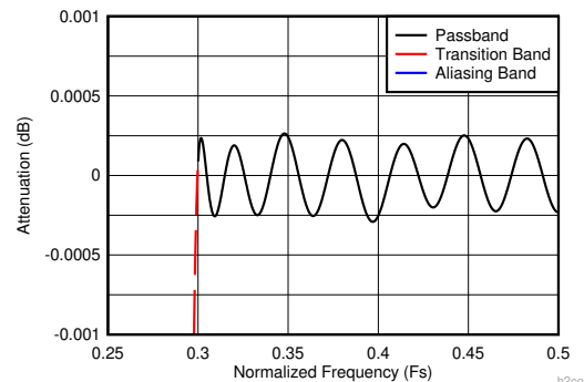
Figure 7-10. Decimate-by-2 Composite Zoomed Pass-Band Response (D2_HIGH_PASS = 1)
