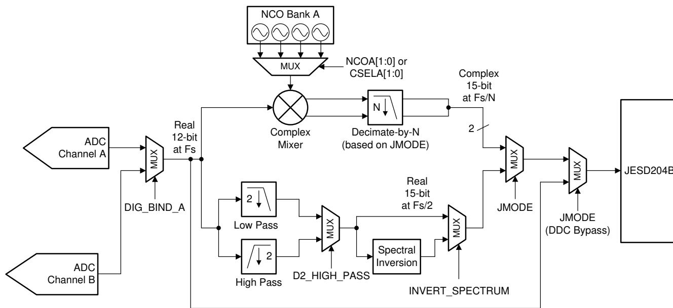
7-5. Channel A Digital Down Conversion Block (Dual-Channel Mode Only)
