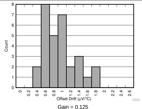
Figure 23. Offset Voltage Drift Distribution
