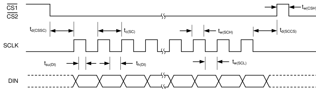
FIG 1. Serial Interface Timing Requirements
