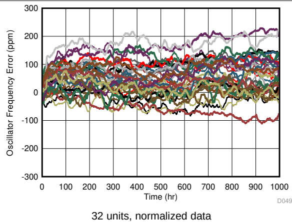
FIG 48. Oscillator Frequency Long-Term Drift
