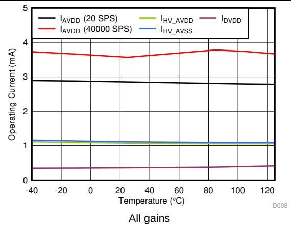
FIG 51. Operating Current vs Temperature
