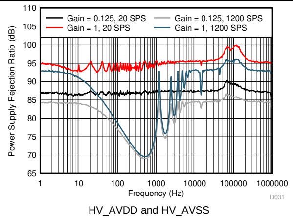
FIG 49. PSRR vs Frequency
