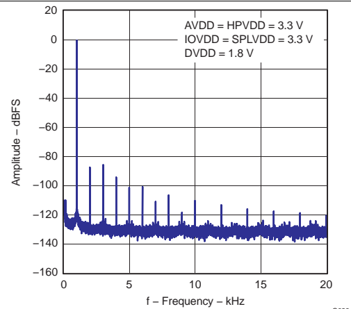
Figure 4-6. Amplitude vs Frequency FFT – DAC to Headphone Output
