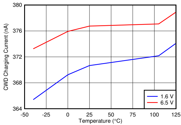
6-4. CWD Charging Current vs Temperature
