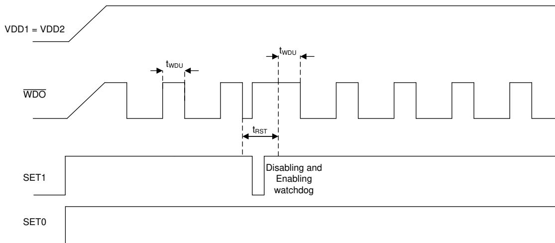
🔗 7-3. Enabling and Disabling the Watchdog Timer During a WDO Reset Event
