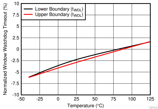
6-6. Normalized Watchdog Timeout Accuracy Over Temperature (SET0 = 1, SET1 = 1, CWD = NC)
