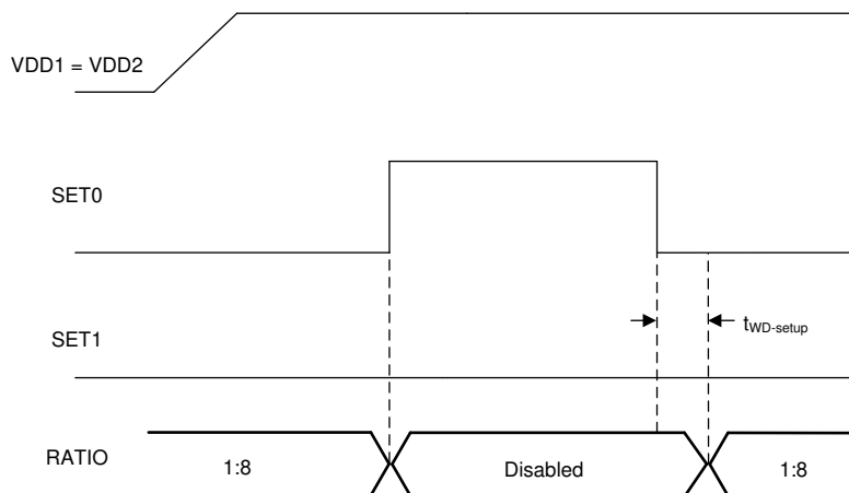
☒ 7-2. Enabling the Watchdog Timer
