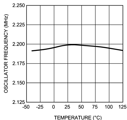
図 5-9. Oscillator Frequency vs Temperature,
