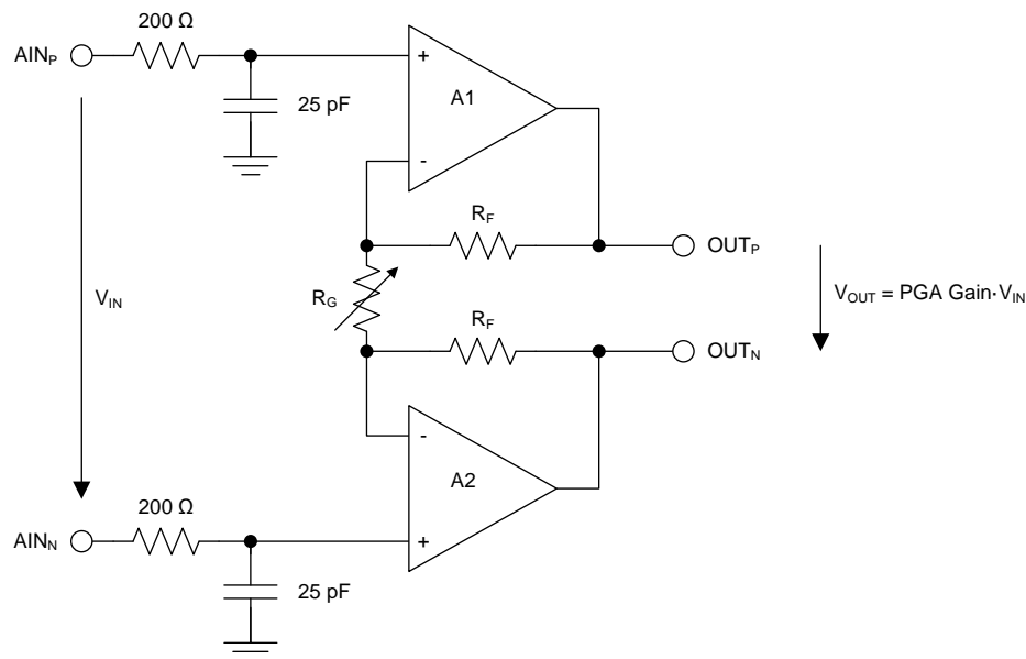
図 43. Simplified PGA Diagram
