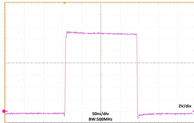
9-1. Switch Node Waveform
