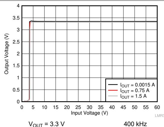
Figure 10-9. Line Regulation
