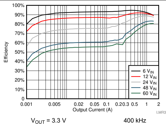
Figure 10-5. Efficiency
