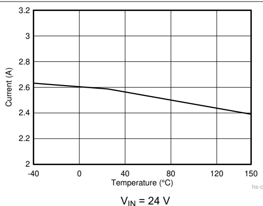
8-3. High Side Current Limit
