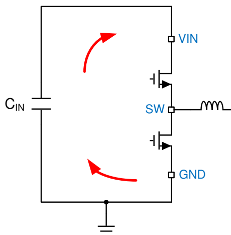
✎ 12-1. Current Loops with Fast Edges
