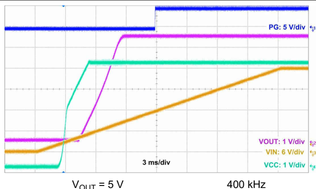
10-14. Start-Up Waveform
