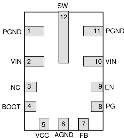
FIG 7-1. 12-Pin VQFN-HR RNX Package (Top View)
