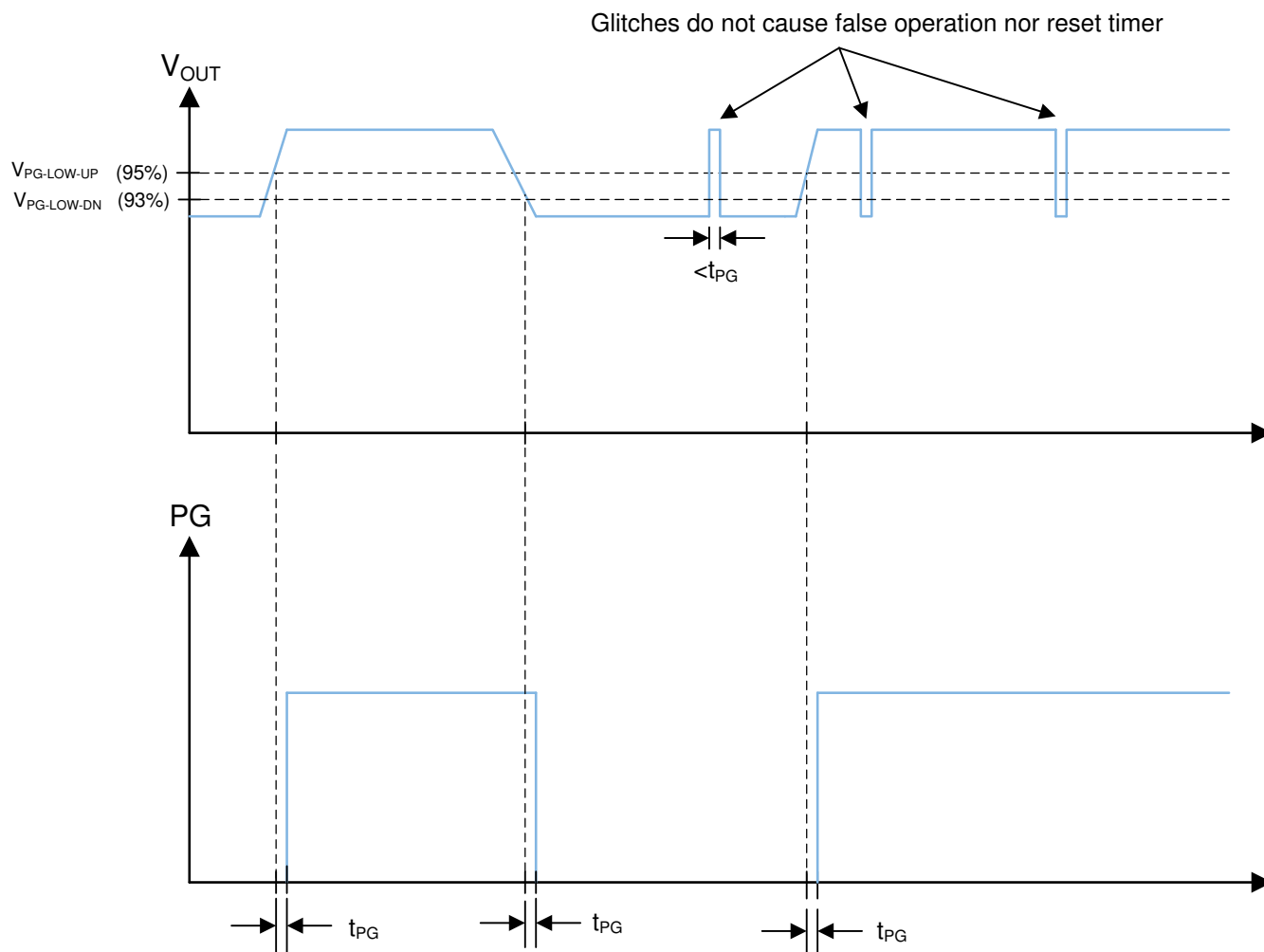
図 9-3. Power-Good-Timing Behavior
