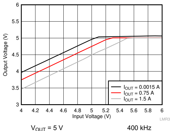
10-10. Overall Dropout Characteristic
