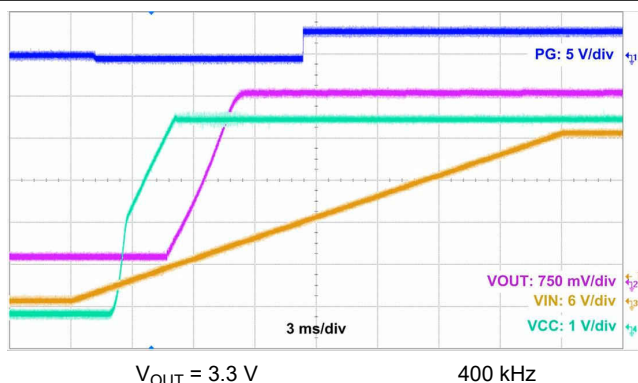
10-15. Start-Up Waveform
