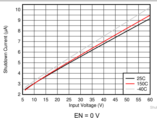
8-2. Shutdown Supply Current
