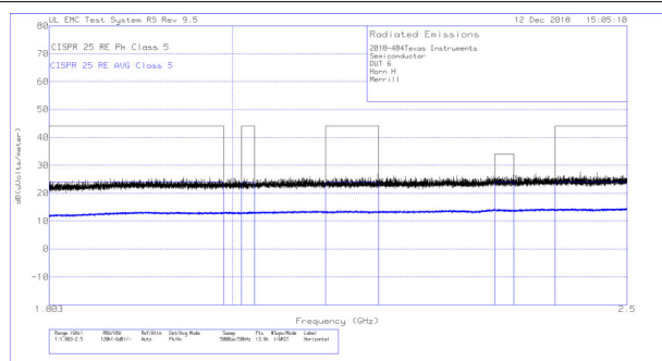
10-24. Radiated EMI Log Horizontal vs. CISPR25 Limits
