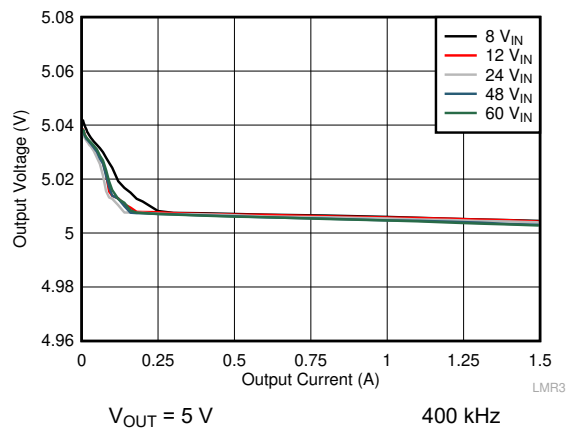
Figure 10-6. Load Regulation
