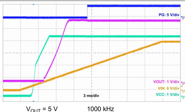
FIG 10-33. Start-Up Waveform
