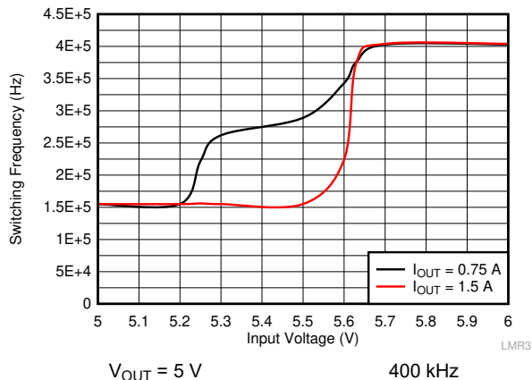
10-11. Frequency Dropout Characteristic
