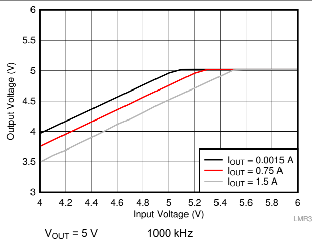
FIG 10-30. Overall Dropout Characteristic
