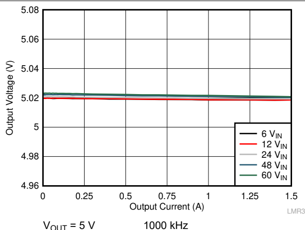
FIG 10-29. Load Regulation
