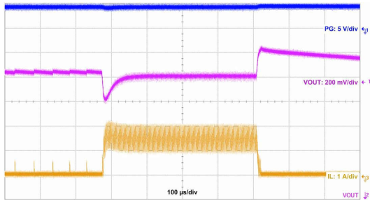
FIG 10-16. Load Transient
