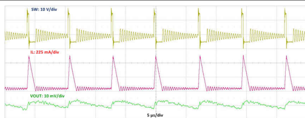
図 9-7. Typical PFM Switching Waveforms V_{IN} = 24 V, V_{OUT} = 5 V, I_{OUT} = 200 mA
