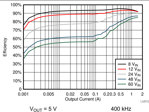
Figure 10-4. Efficiency
