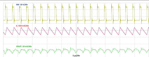
図 9-8. Typical PWM Switching Waveforms V_{IN} = 24 V, V_{OUT} = 5 V, I_{OUT} = 1.5 A, f_s = 400 kHz
