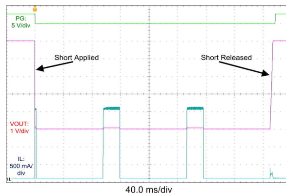
図 9-6. Short-Circuit Transient and Recovery
