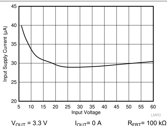
10-12. Input Supply Current
