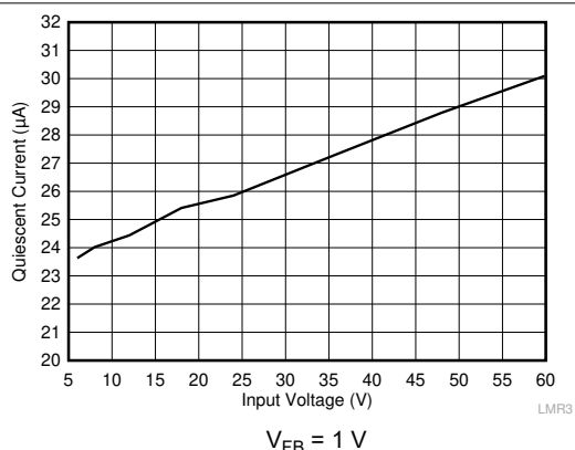
8-1. Non-Switching Input Supply Current
