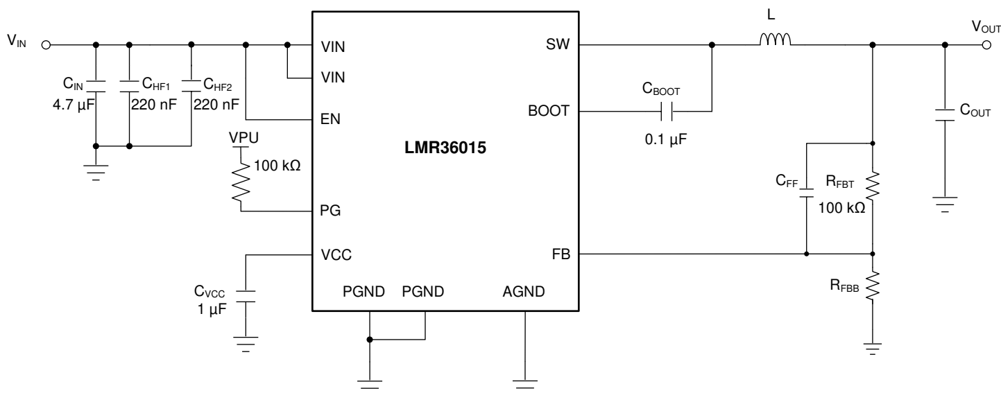
☒ 10-1. Example Applications Circuit
