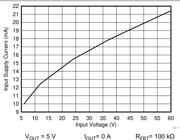
FIG 10-32. Input Supply Current
