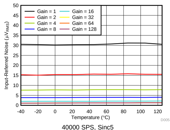
FIG 20. Noise vs Temperature
