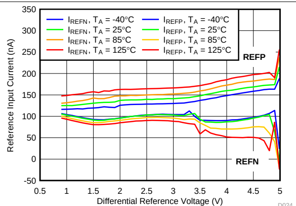
I_{REFP} measured with V_{REFN} = AVSS I_{REFN} measured with V_{REFP} = AVDD
