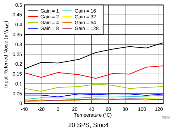
FIG 18. Noise vs Temperature
