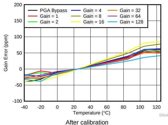
FIG 15. Gain Error vs Temperature
