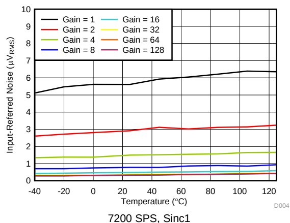
FIG 19. Noise vs Temperature
