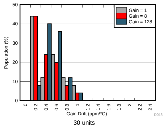
FIG 16. Gain Error Drift Distributions
