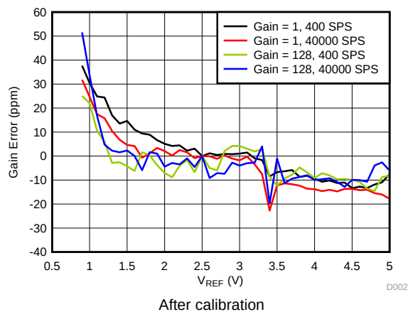
FIG 17. Gain Error vs Reference Voltage
