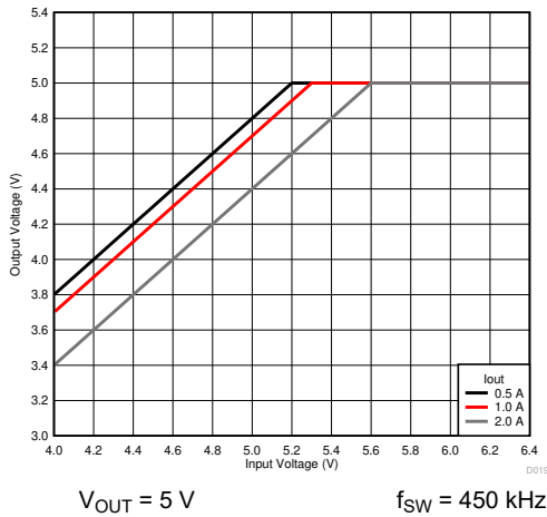
7-4. Voltage Dropout
