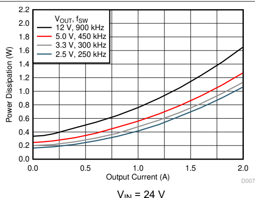
6-10. Power Dissipation vs Output Current
