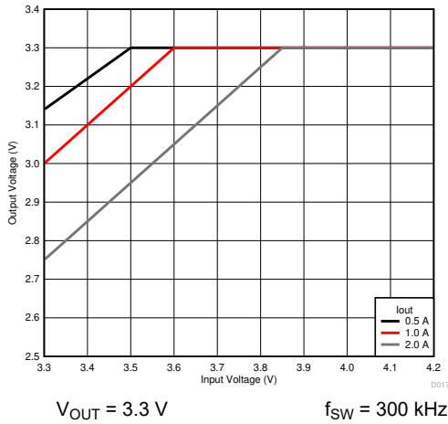
7-2. Voltage Dropout
