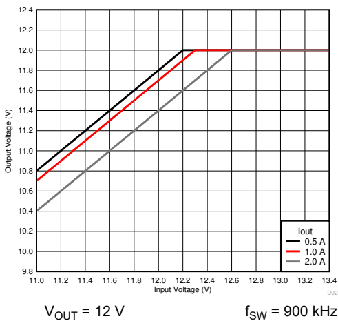
7-6. Voltage Dropout
