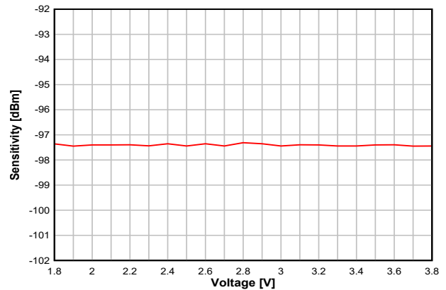
図 8-15. Sensitivity vs. Supply Voltage (VDD) (BLE 1 Mbps, 2.44 GHz, DCDC Off)
