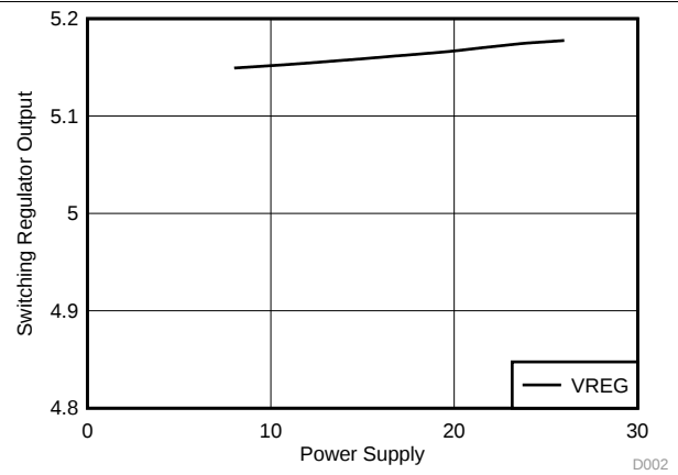
Figure 2. Step-down Regulator Output vs Power Supply (V regSel = 0)
