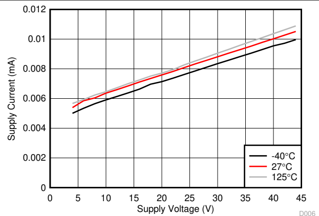
Figure 7-6. Standby Recessive I_{SUP} vs V_{SUP} and Temperature
