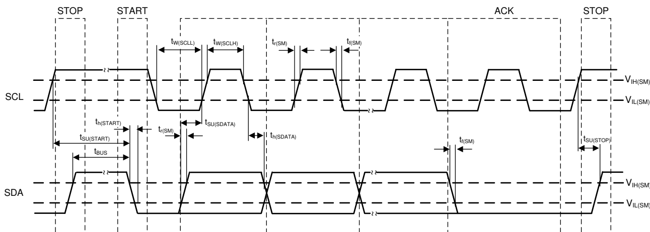
❏ 8-5. I 2 C Timing Diagram
