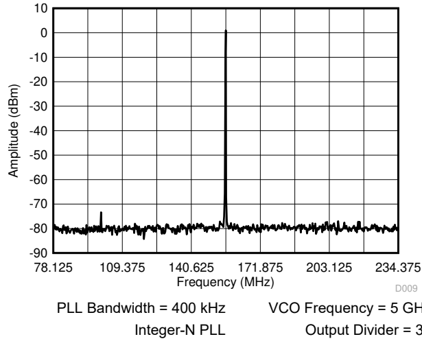
6-9. 156.25 ± 78.125-MHz HCSL Differential Output Spectrum
