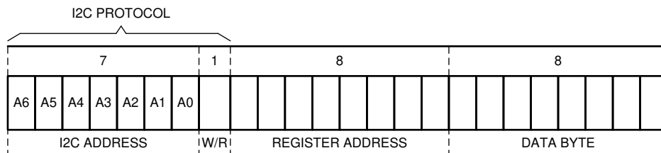
8-6. I 2 C Register Structure
