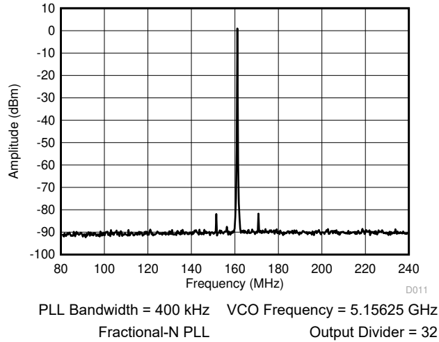
6-11. 161.1328125 ± 80.56640625-MHz LVDS Output Spectrum
