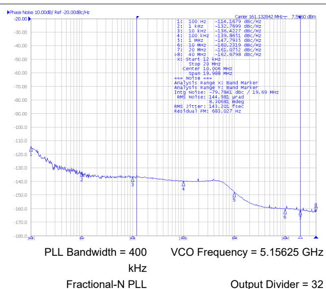
Figure 6-4. Closed-Loop Phase Noise of LVPECL Differential Output at 161.1328125 MHz
