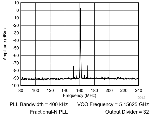
6-12. 161.1328125 ± 80.56640625-MHz HCSL Output Spectrum
