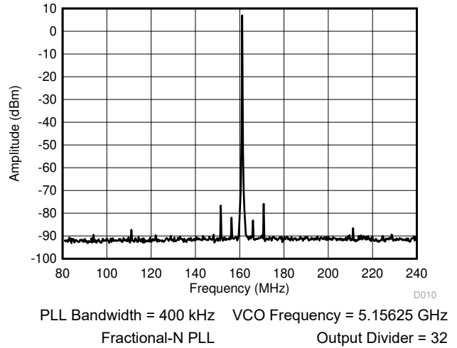
6-10. 161.1328125 ± 80.56640625-MHz LVPECL Differential Output Spectrum
